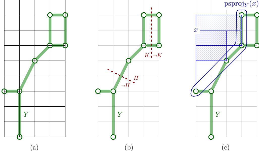
FIGURE 2. (a) A median subalgebra Y (circled vertices) of a grid median graph, and the edges of the corresponding median graph on that subalgebra (thick lines); together with (b) two hyperplanes (dashed lines) within Y ; and (c) the pseudoprojection (Proposition 2.14) of a vertex x onto Y , and all minimal intervals between them.
