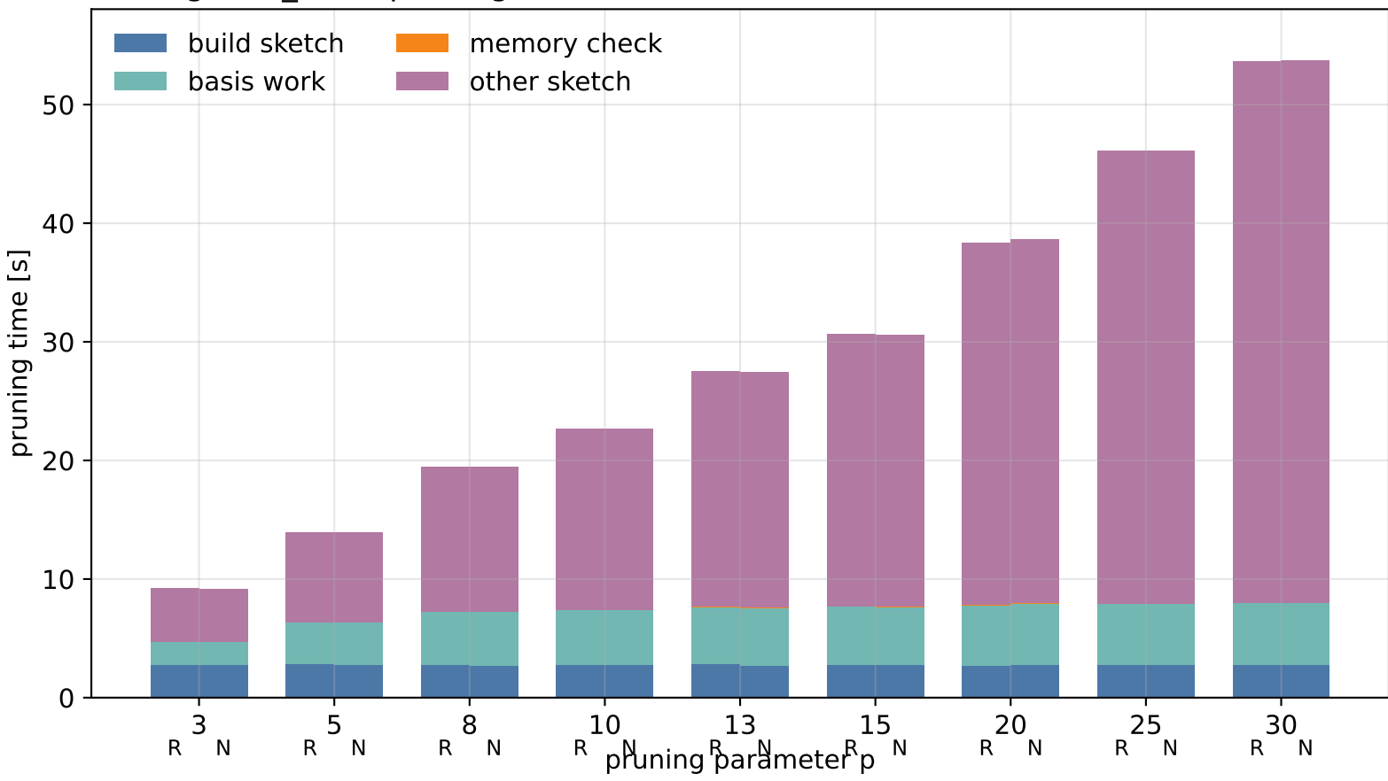
gf2^8_mult: pruning-time breakdown (R: with reuse, N: without reuse)
