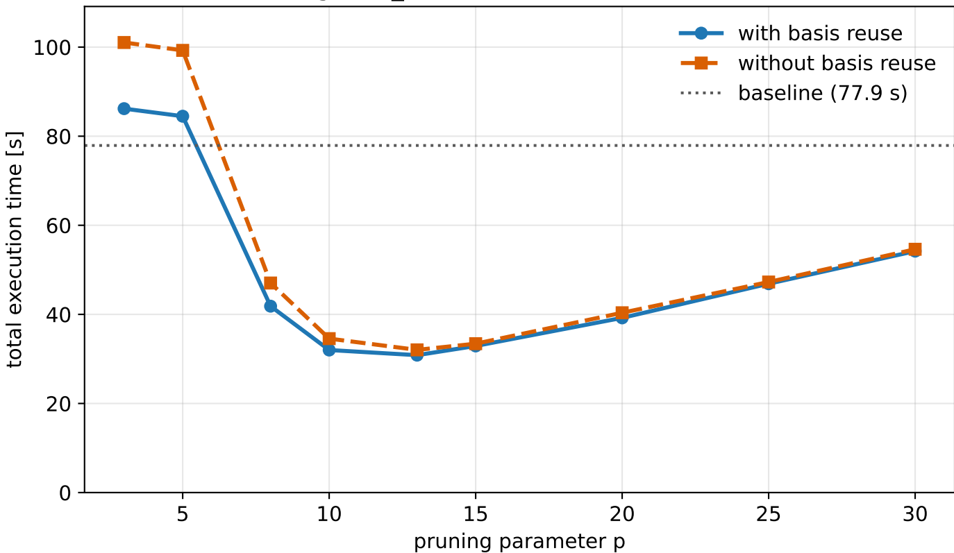
gf2^8_mult: total execution time
