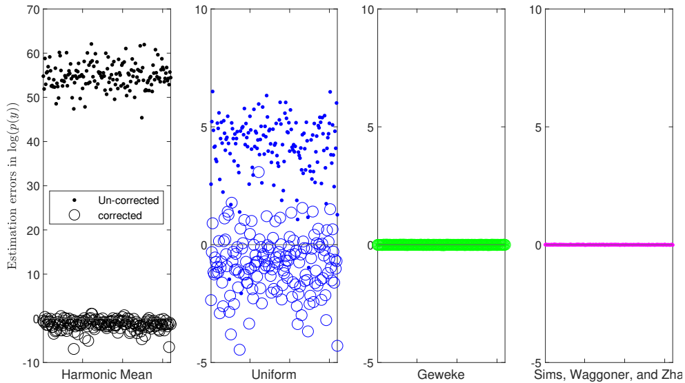
Figure C.1: Estimation errors in a Bayesian linear regression model
