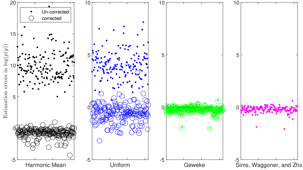
Figure C.2: Estimation errors in a small-scale DSGE model
