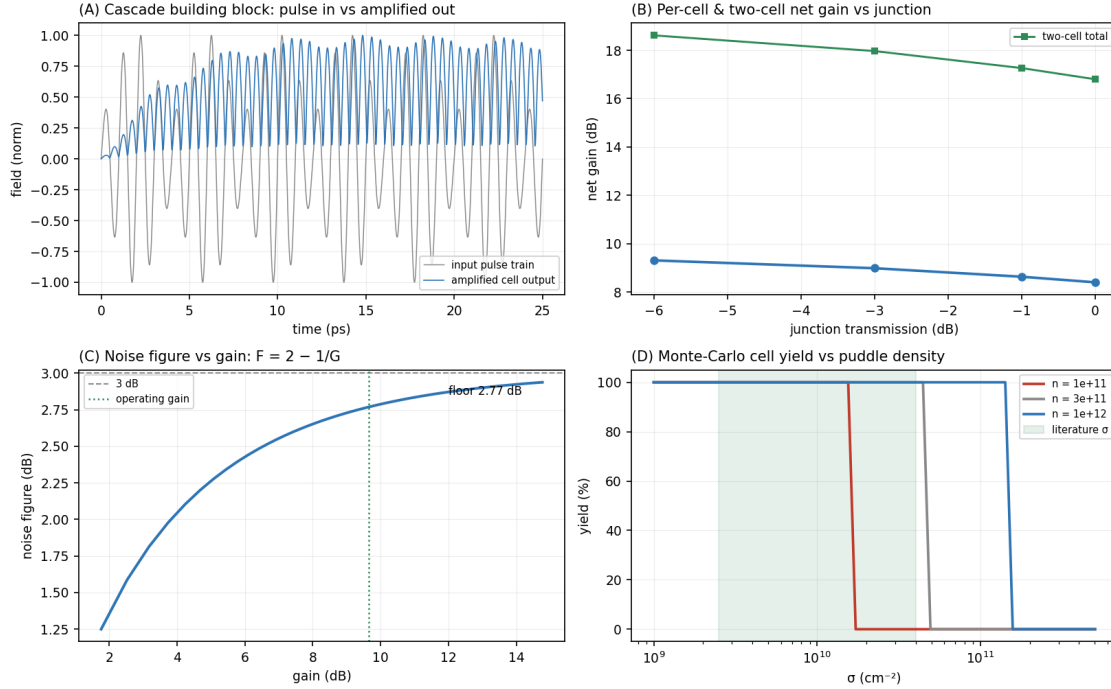
Figure 9. Pass 4. (A) Cascade building block: the input pulse train and the amplified cell output (solver). (B) Per-cell and two-cell net gain vs junction transmission — per-cell gain rises as junction loss unloads the saturating rail. (C) Noise figure F = 2 - 1/G vs gain; floor \approx 2.8 dB at the operating gain. (D) Monte-Carlo cell yield vs puddle density \sigma , with the literature range shaded; n = 10^{12} clears it with margin.
