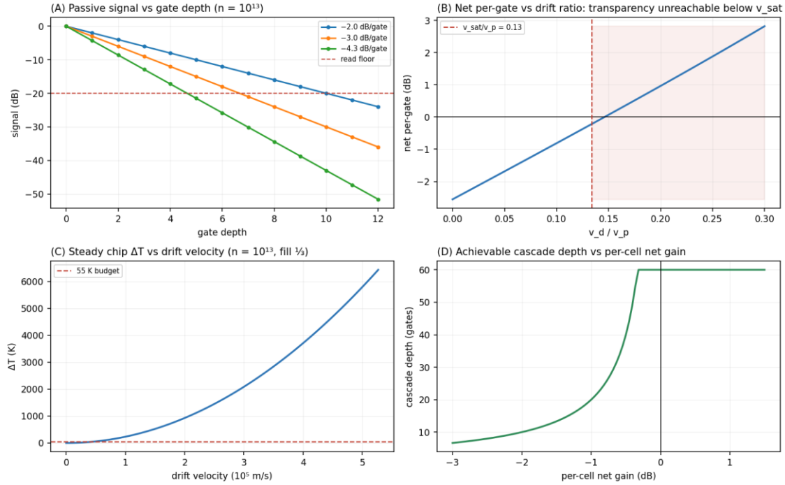
Figure 6. Pass 1, at n = 10^{13} \text{ cm}^{-2} and 353 K. (A) Passive signal vs gate depth for the candidate per-gate budgets. (B) Net per-gate result vs drift ratio v_d/v_p : transparency is unreachable below v_{\text{sat}} . (C) Steady-state chip \Delta T vs drift velocity against the 55 K budget. (D) Achievable cascade depth vs per-cell net gain. Per-gate loss convention: one \lambda_p/2 of propagation (Appendix A).
