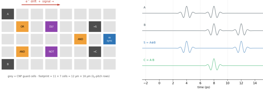
(b) Cell map on the gate lattice (one re-sync segment; drift and signal →, co-propagating) Slot-level timing: pipelined at 0.25 THz (one addition per 4-ps slot; latency = 1 ps, sub-slot)
