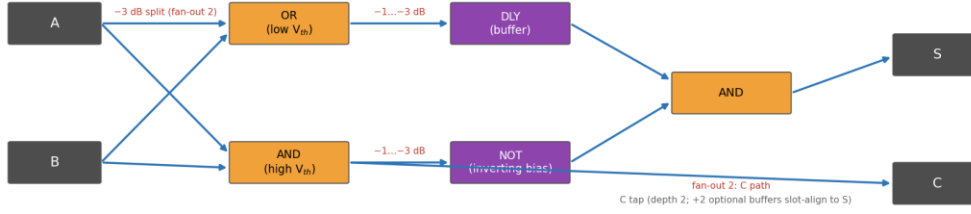
(a) The half adder netlist: 5-cell regenerative core (+2 optional C-alignment buffers)
