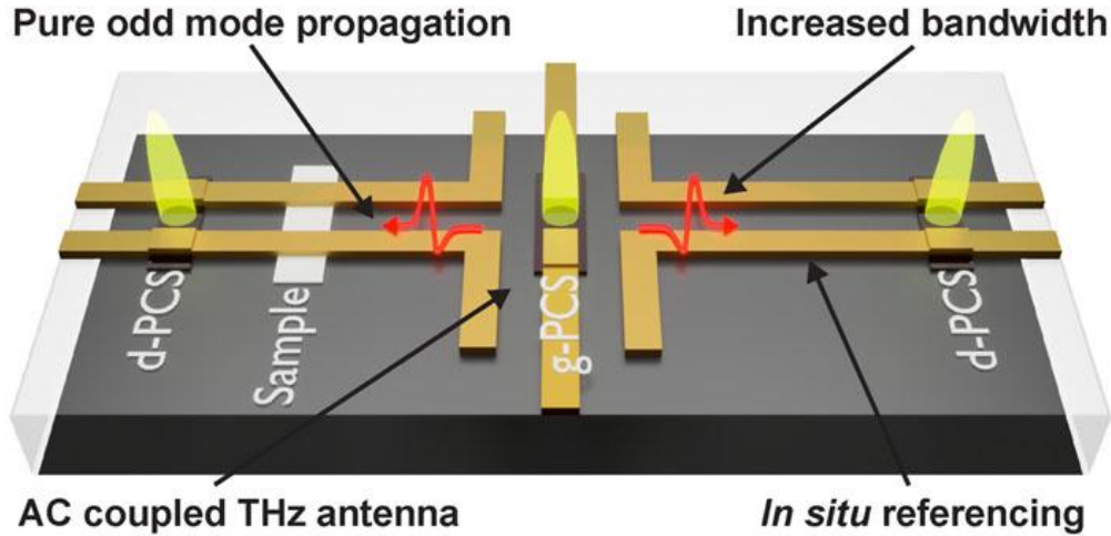
Figure 2. Monolithic launcher/detector/reference circuit, reproduced from Kusyak et al. [7] (CC BY-NC 4.0): APL Photonics 10, 076117 (2025): generator switch ( g -PCS) centered on a coplanar stripline with two symmetric detector switches ( d -PCS) — galvanic isolation plus in-situ referencing. Used at the fabric edges for launch/read-out and reused mid-fabric as re-sync clock taps.
