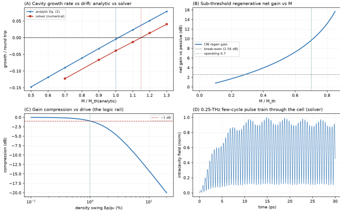
Figure 8. Pass 3 (coarse-grid Lax-Friedrichs M_{\text{th,num}} \approx 0.169 — inviscid limit \approx 0.149 , physical kinetic threshold 0.165; operating ratio M/M_{\text{th,num}} = 0.7 ). (A) Cavity growth rate vs drift, analytic Eq. (2) vs the nonlinear solver, both thresholds marked — the solver's numerical diffusion shifts its threshold \sim 15 % higher. (B) Sub-threshold CW regenerative net gain vs M ; break-even at the per-gate ( \lambda_p/2 ) loss; +9.7 dB at the working ratio. (C) Gain compression vs drive amplitude — the logic rail (1 dB at \approx 1 % swing). (D) The 0.25 THz few-cycle pulse train building up in the cell (solver, intracavity field).
