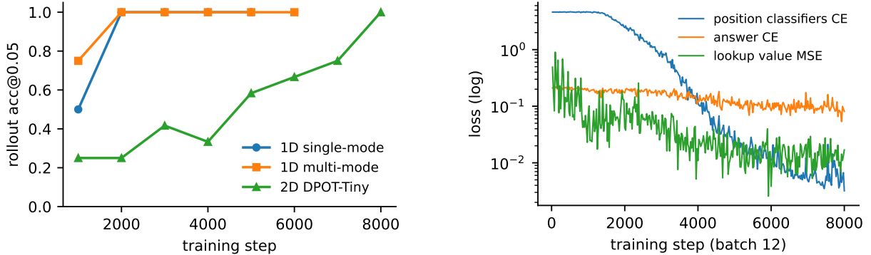
Figure 3: Left: rollout accuracy per training chunk for the three \Psi LM configurations. Right: 2D training phase structure — the four positional classifiers lock in first (over \sim 5k steps); the answer loss converges only after the pointer does, echoing Stage 1’s causal ordering.
