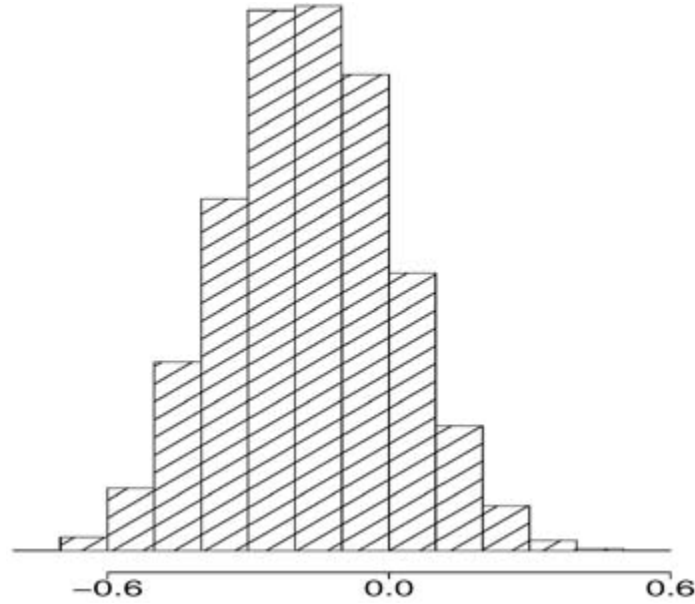
FIGURE 24.1. Posterior of \delta from simulation.
