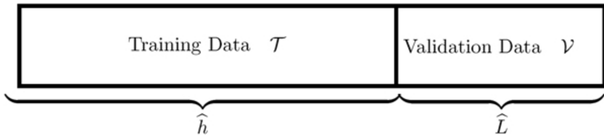
FIGURE 22.6. Cross-validation. The data are divided into two groups: the training data and the validation data. The training data are used to produce an estimated h classifier \hat{h} . Then, \hat{h} is applied to the validation data to obtain an estimate \hat{L} of the error rate of \hat{h} .
