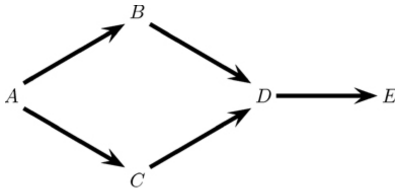
FIGURE 17.4. Yet another DAG.
