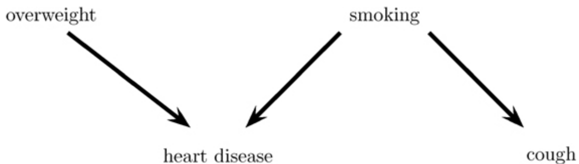
FIGURE 17.2. DAG for Example 17.4.
