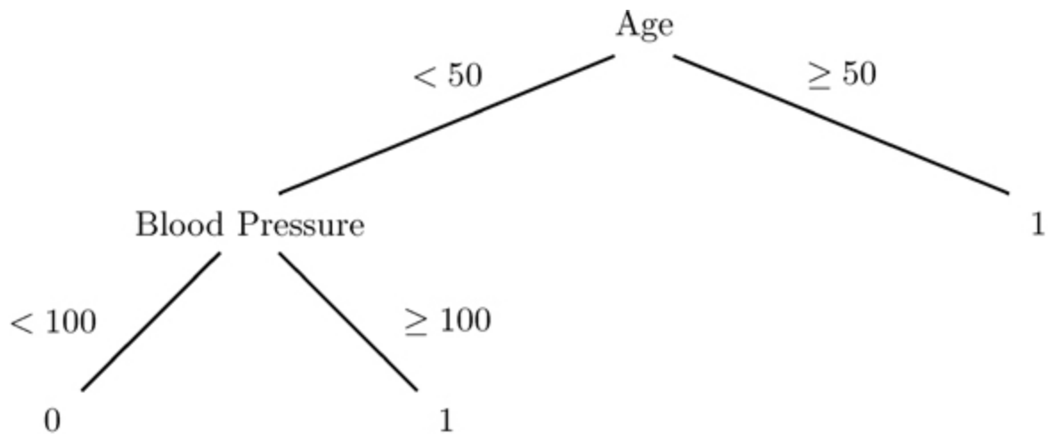
FIGURE 22.2. A simple classification tree.
