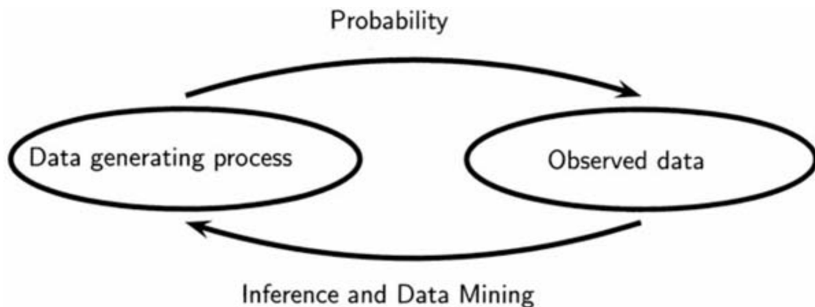
FIGURE 1. Probability and inference.
