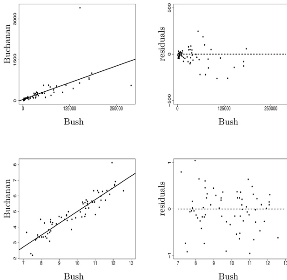
Figure 13.2. Voting Data for Election 2000. See example 13.6 .
