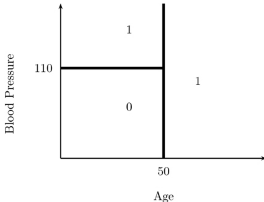
FIGURE 22.3. Partition representation of classification tree.
