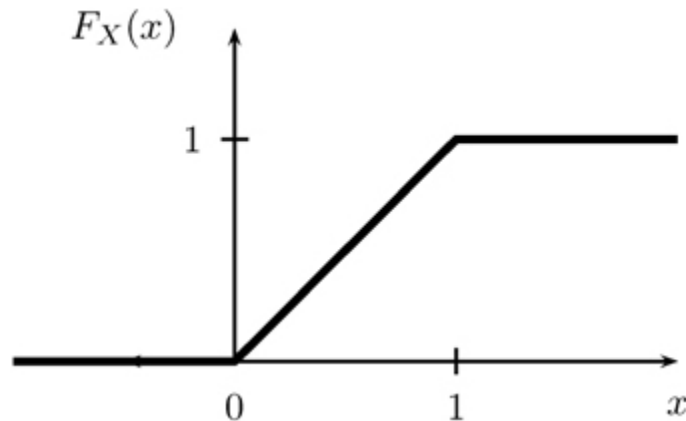
FIGURE 2.3. CDF for Uniform (0, 1).
