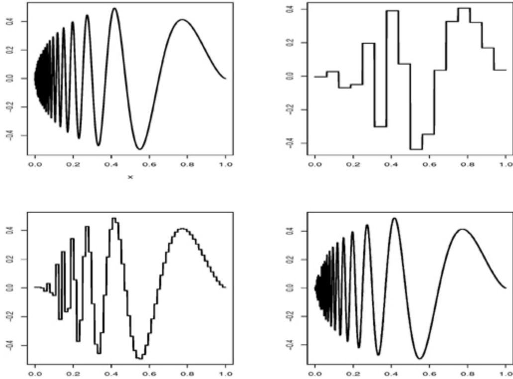
FIGURE 21.7. The doppler signal and its reconstruction
