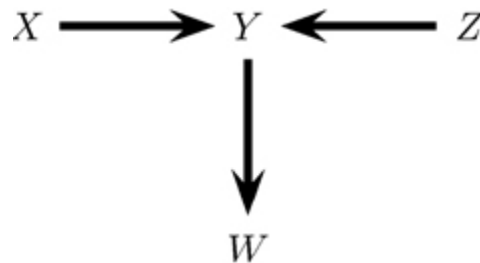
FIGURE 17.7. A collider with a descendant.
