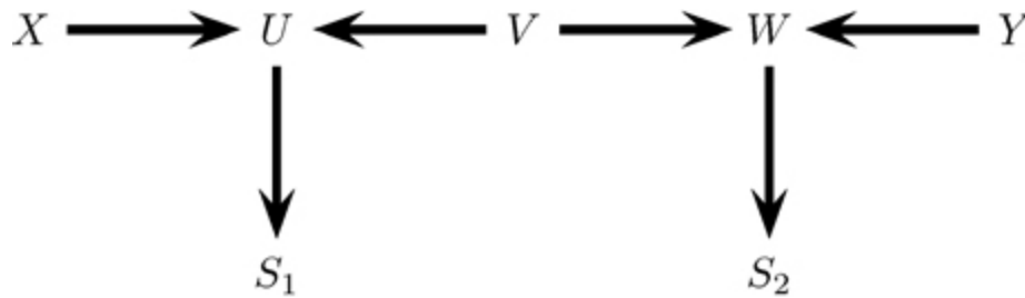
FIGURE 17.8. d-separation explained.
