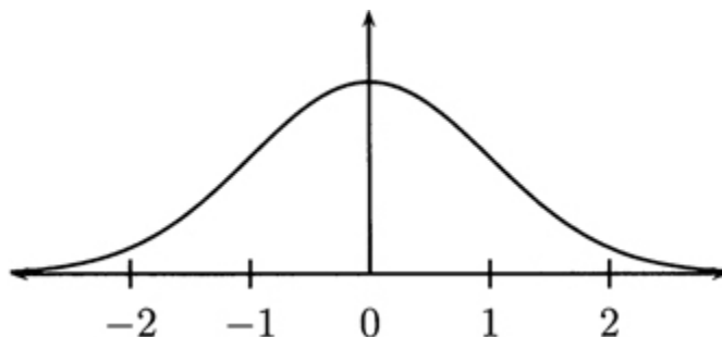
FIGURE 2.4. Density of a standard Normal.
