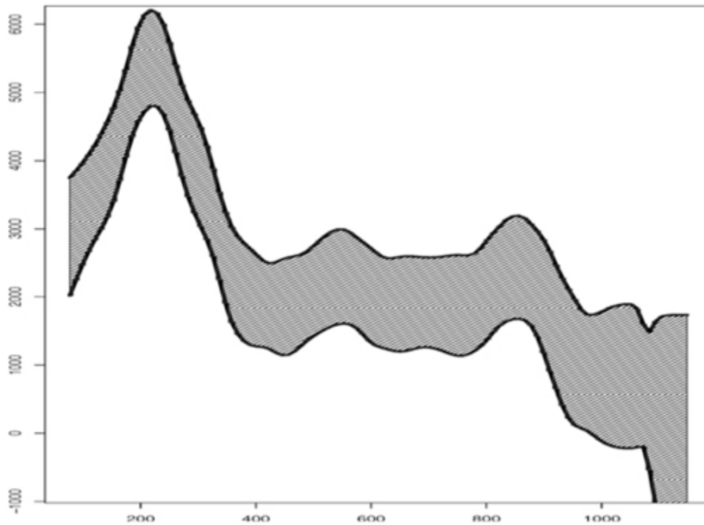
FIGURE 20.9. 95 percent confidence envelope for the CMB data.
