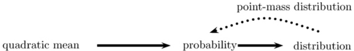
FIGURE 5.2. Relationship between types of convergence.
