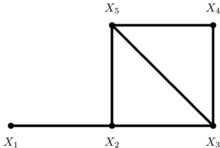
FIGURE 19.1. Graph for Example 19.7 .
