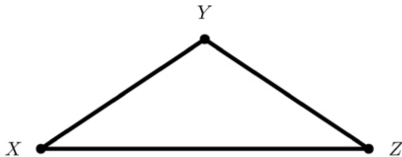
Figure 18.4. No implied independence relations.
