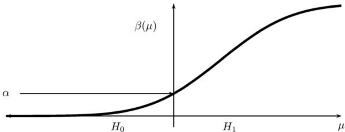
FIGURE 10.1. The power function for Example 10.2 . The size of the test is the largest probability of rejecting H_0 when H_0 is true. This occurs at \mu = 0 hence the size is \beta(0) . We choose the critical value c so that \beta(0) = \alpha .
