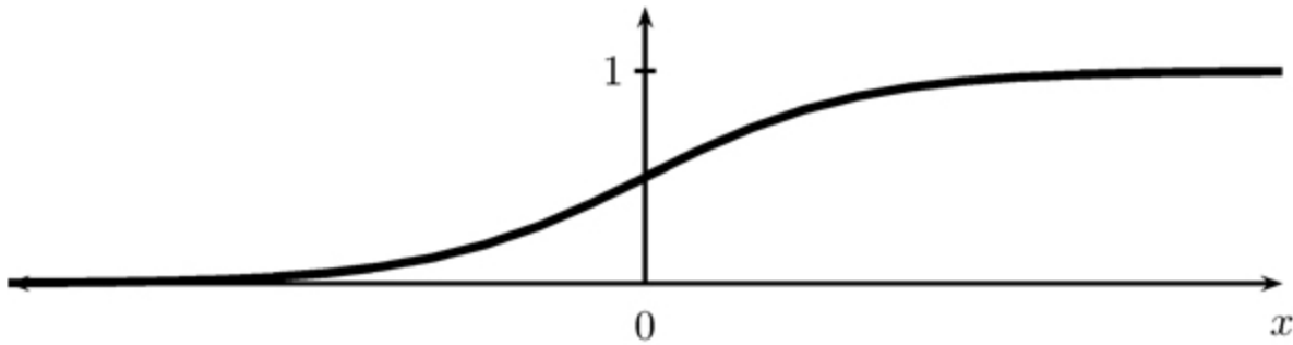
Figure 13.3. The logistic function p = e^x/(1 + e^x) .
