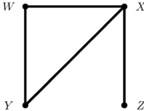
Figure 18.2. \{Y, W\} and \{Z\} are separated by \{X\} . Also, W and Z are separated by \{X, Y\} .
