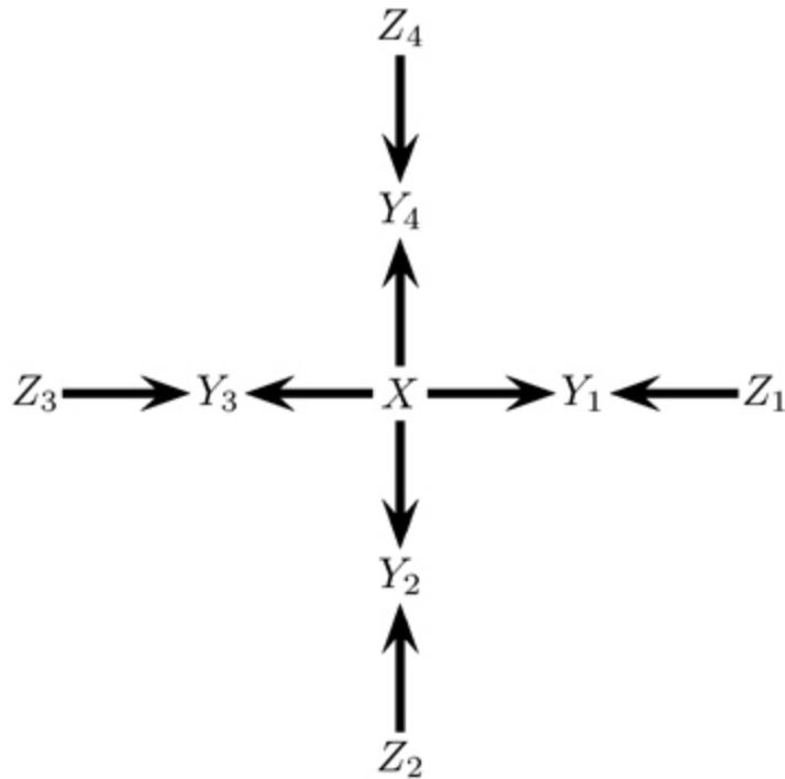
FIGURE 17.12. DAG for exercise 7.
