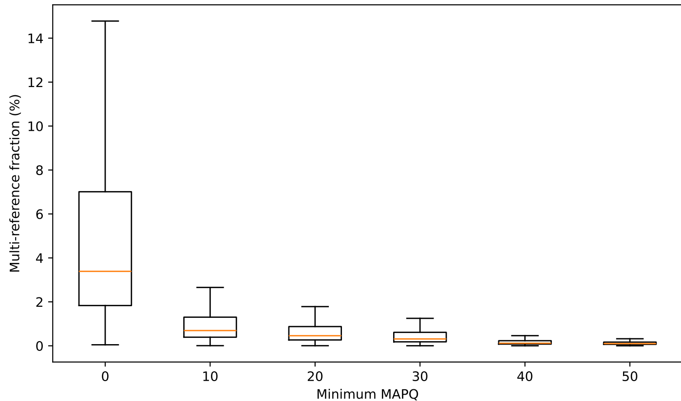
Silene latifolia : nuclear-organelle ambiguity across MAPQ
