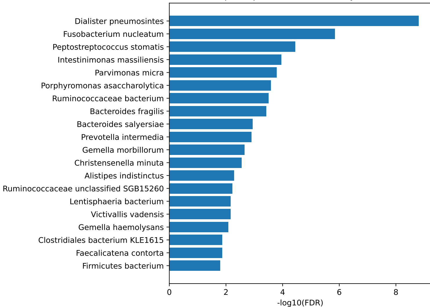
Top 20 species: Mann-Whitney U test
