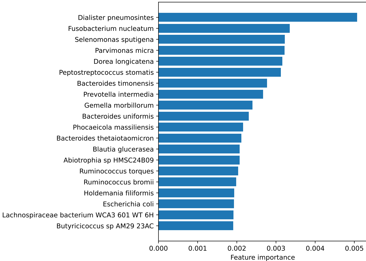
Top 20 features: Extra Trees
