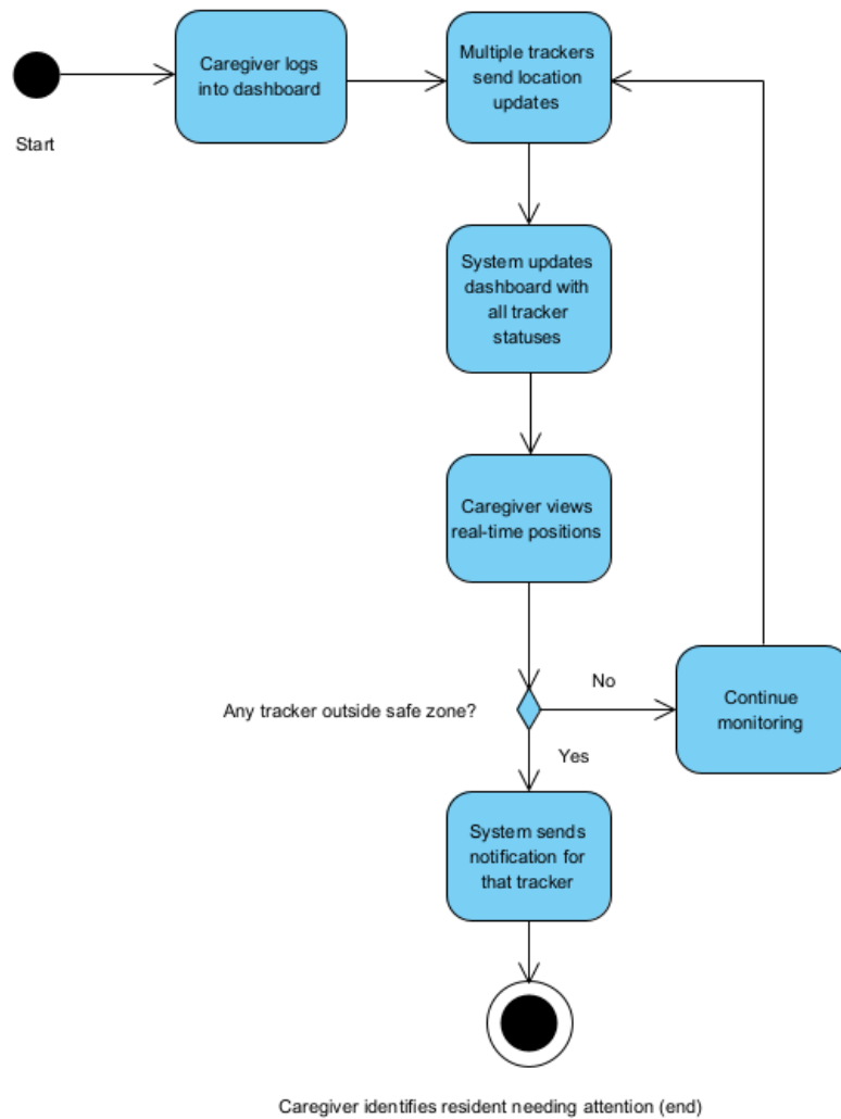
Figure 6.4: ucMultiResidentMonitoringActivity: Activity Diagram for Multi-Resident Monitoring (UC2)
