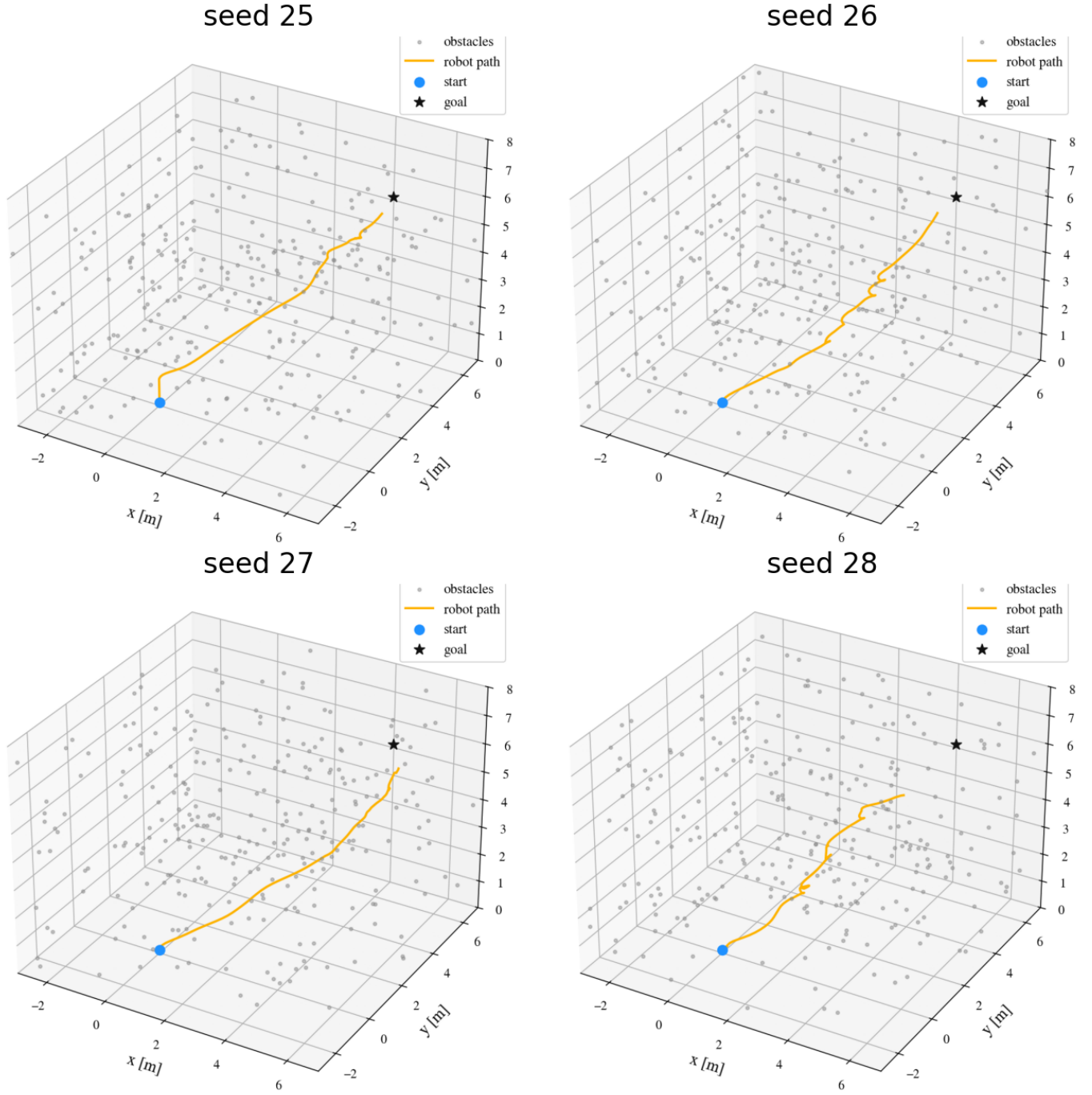
Fig. 6. Closed-loop FCP-MPC trajectories in the dense 3D quadrotor task across four random seeds ( M=280 dynamic obstacles, seeds 25–28). Blue dot: start; black star: goal; gray points: dynamic-obstacle positions at episode end. FCP-MPC navigates through the dense environment in each seed, demonstrating consistent progress toward the goal despite heavy obstacle density.
