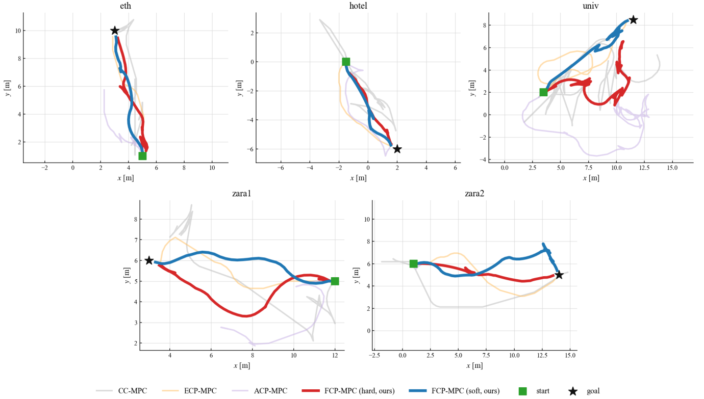
Fig. 3. Representative closed-loop trajectories on one scene of each of the five ETH-UCY datasets (green squares: start; black stars: goal). Both variants of FCP-MPC (ours)—soft (thick blue) and hard (thick red)—reach the goal along direct paths, whereas the baselines, drawn in lighter lines, tend to wander or stall: CC-MPC (gray) is slow and conservative, ECP-MPC (orange) detours, and ACP-MPC (purple) often fails to make steady progress in dense scenes such as univ.
