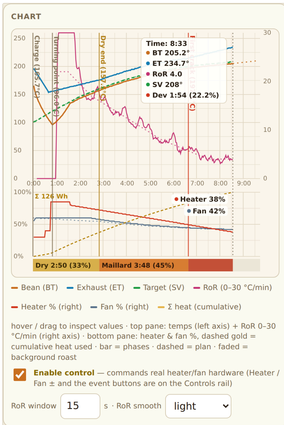
Fig. 10 — Just before Drop at 8:30. First Crack is marked and the development phase is shown on the bar.
