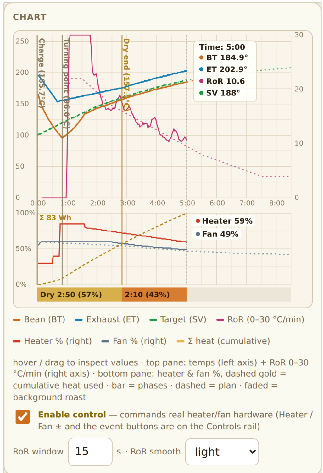
Fig. 9 — The chart at 5:00 with Charge, turning point and Dry End marked. Hover or drag to read values. Below the chart: the Enable control tick and the RoR settings.
