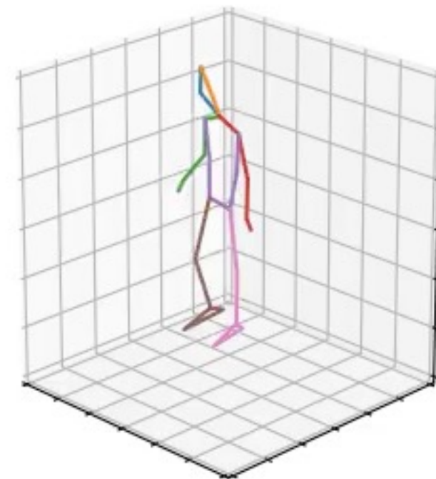
ground truth
