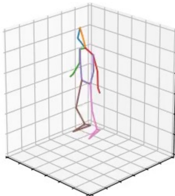
prediction
