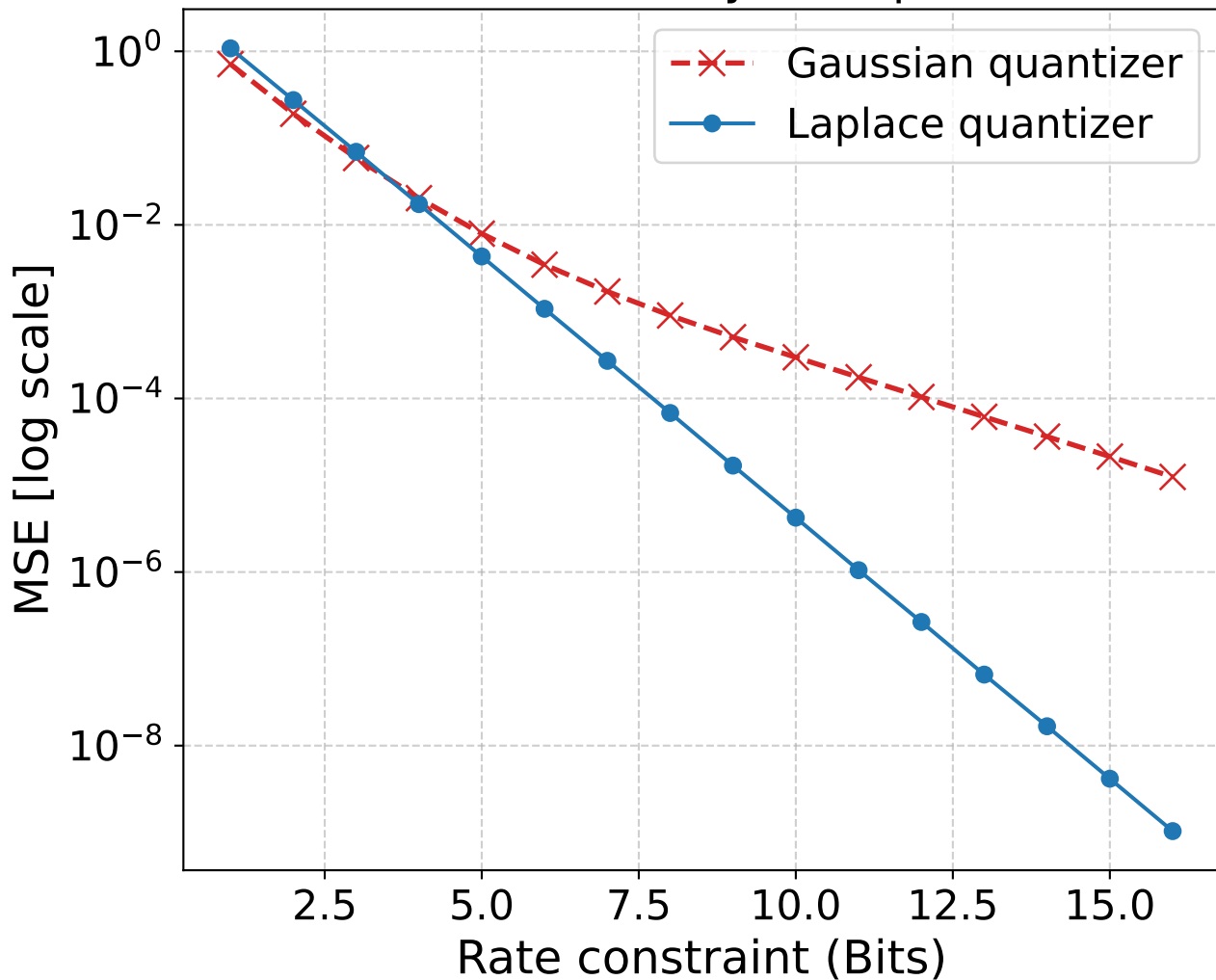
Quantization efficiency on Laplace source
