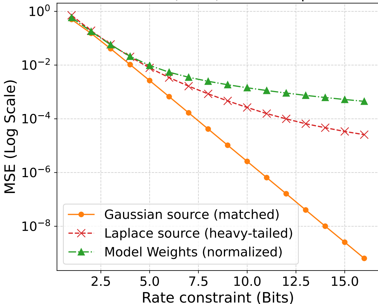
Panter & Dite (1951) Gaussian quantizer
