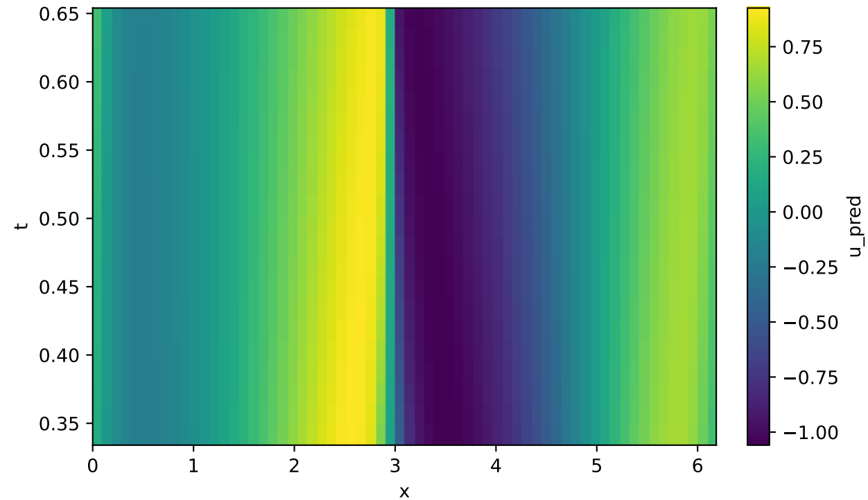
Predicted u(t,x)
