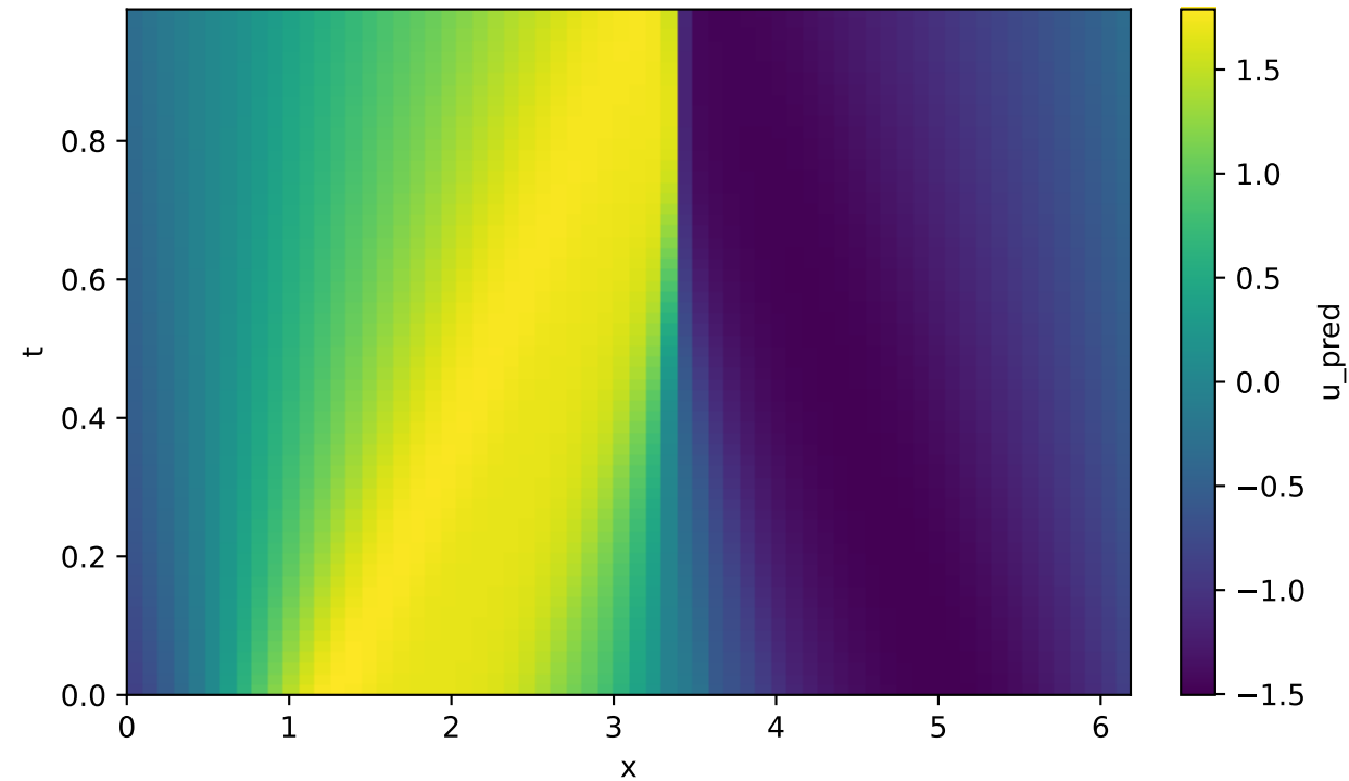
Predicted u(t,x)
