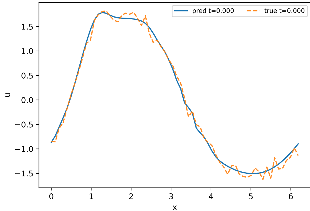
Snapshots: pred vs true
