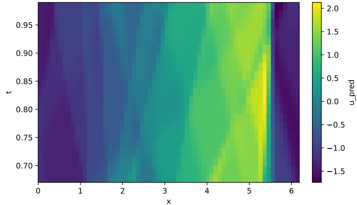
Predicted u(t,x)
