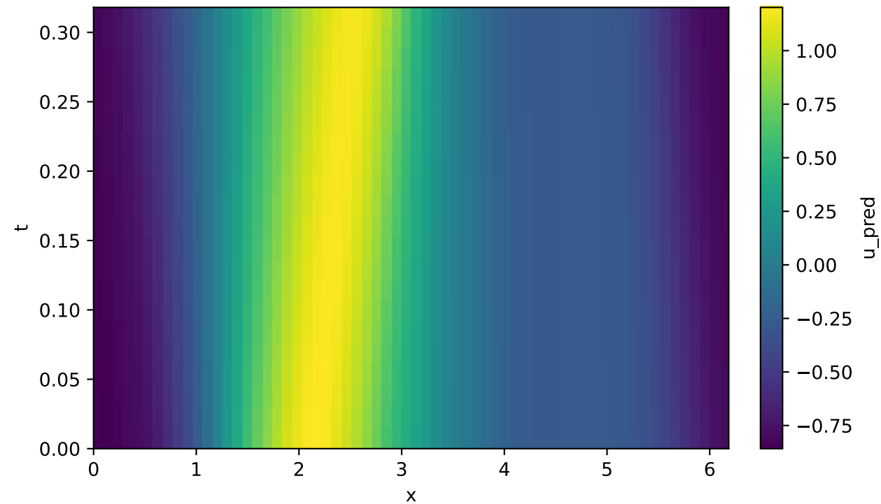
Predicted u(t,x)
