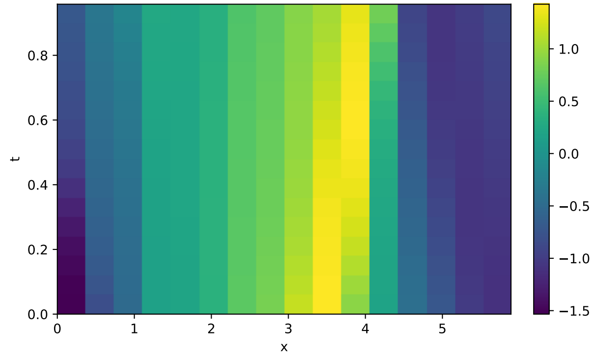
Predicted u(t,x)
