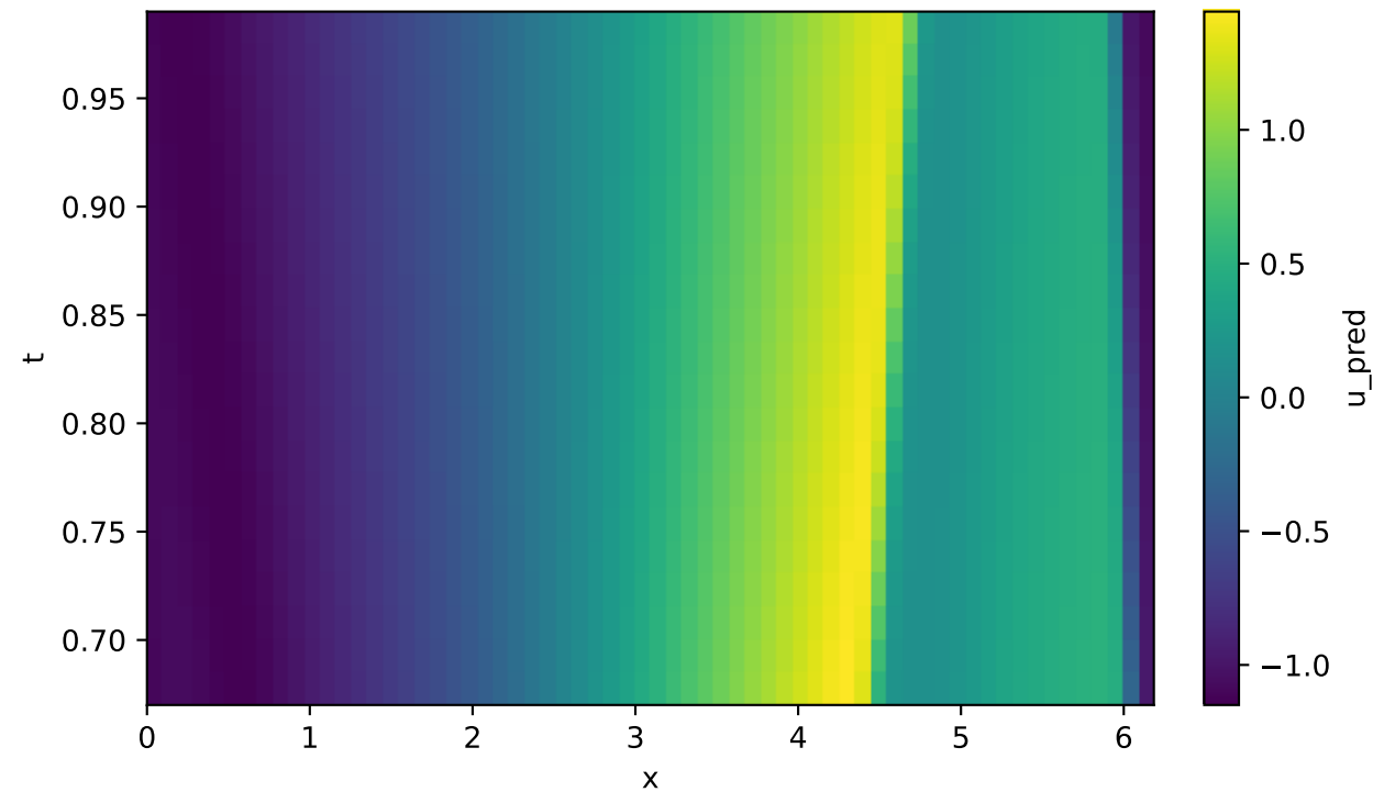
Predicted u(t,x)
