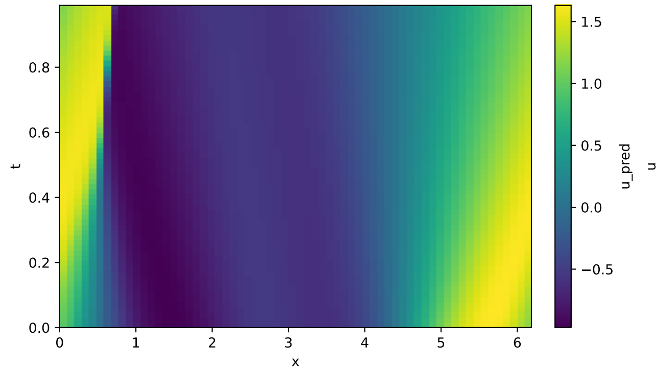
Predicted u(t,x)
