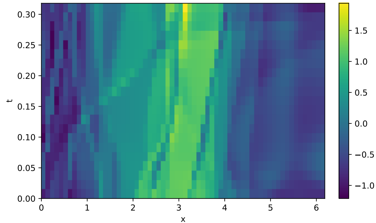
Predicted u(t,x)
