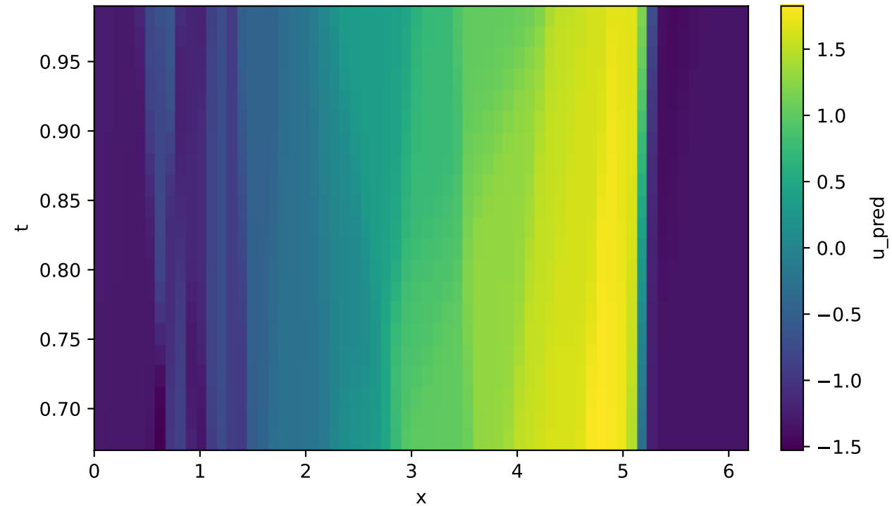
Predicted u(t,x)
