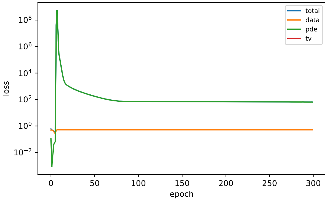
pde_lambda=0.5 seed=1
