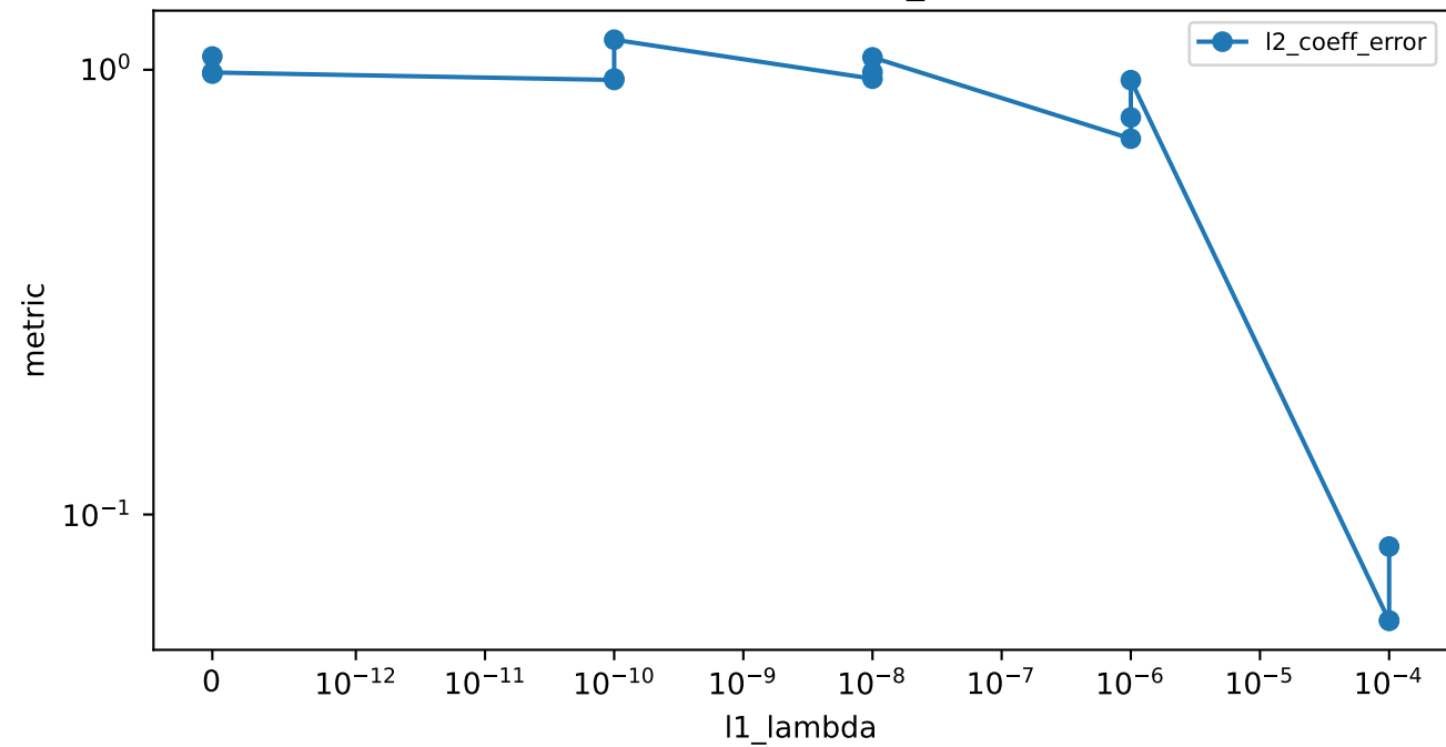
PDE coeff error vs l1_lambda
