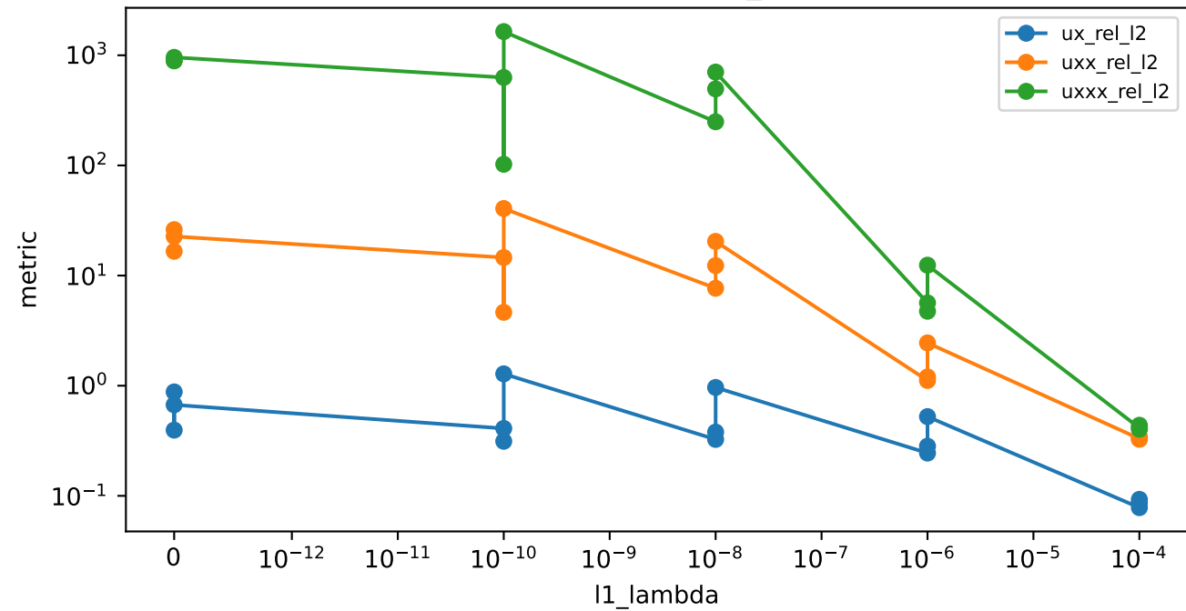
derivative error vs l1_lambda
