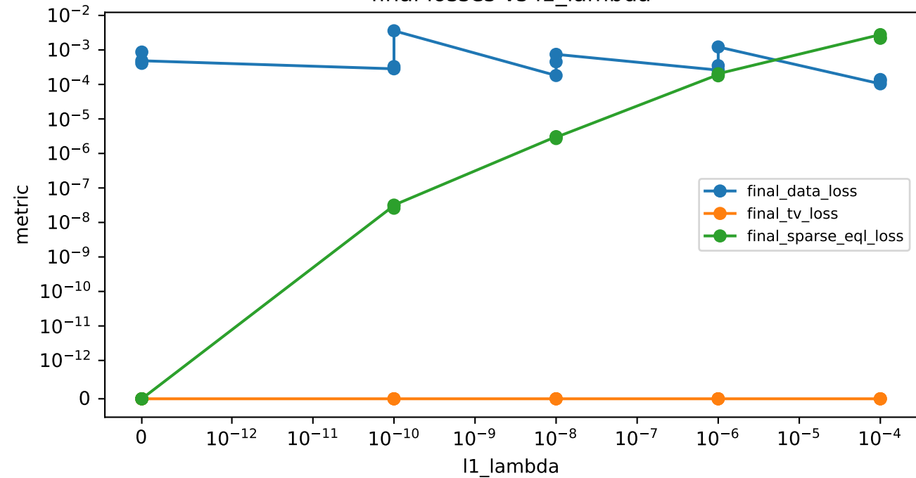
final losses vs l1_lambda
