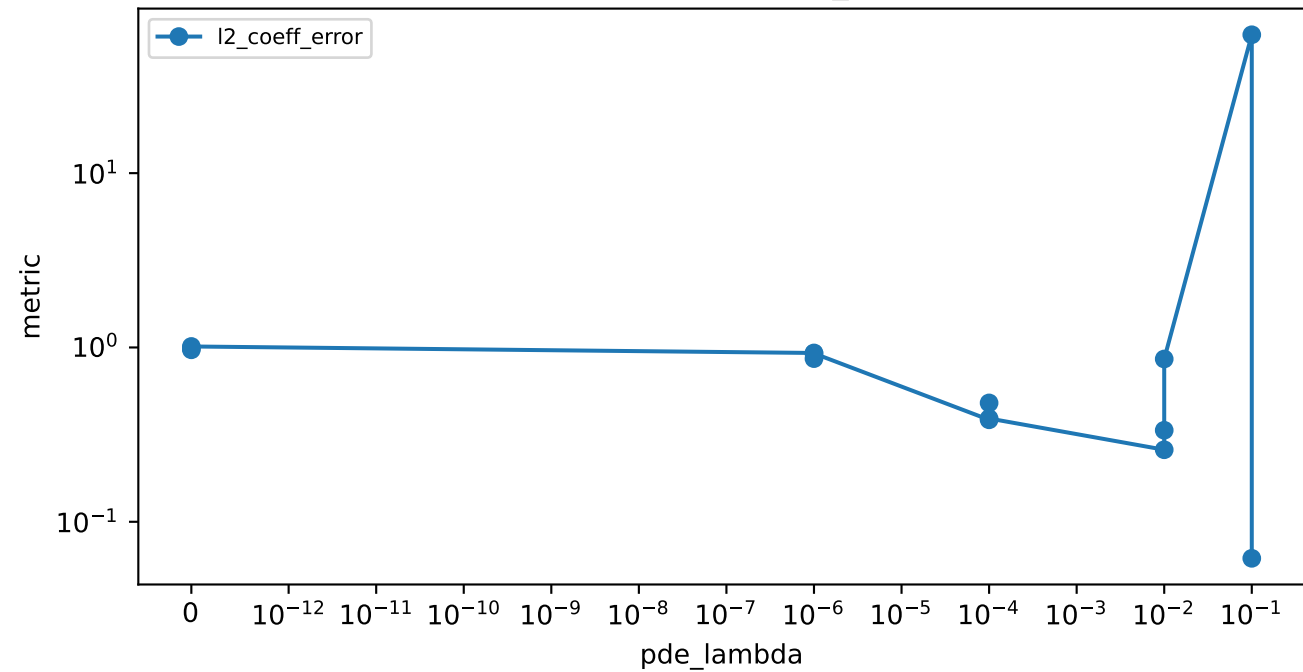
PDE coeff error vs pde_lambda
