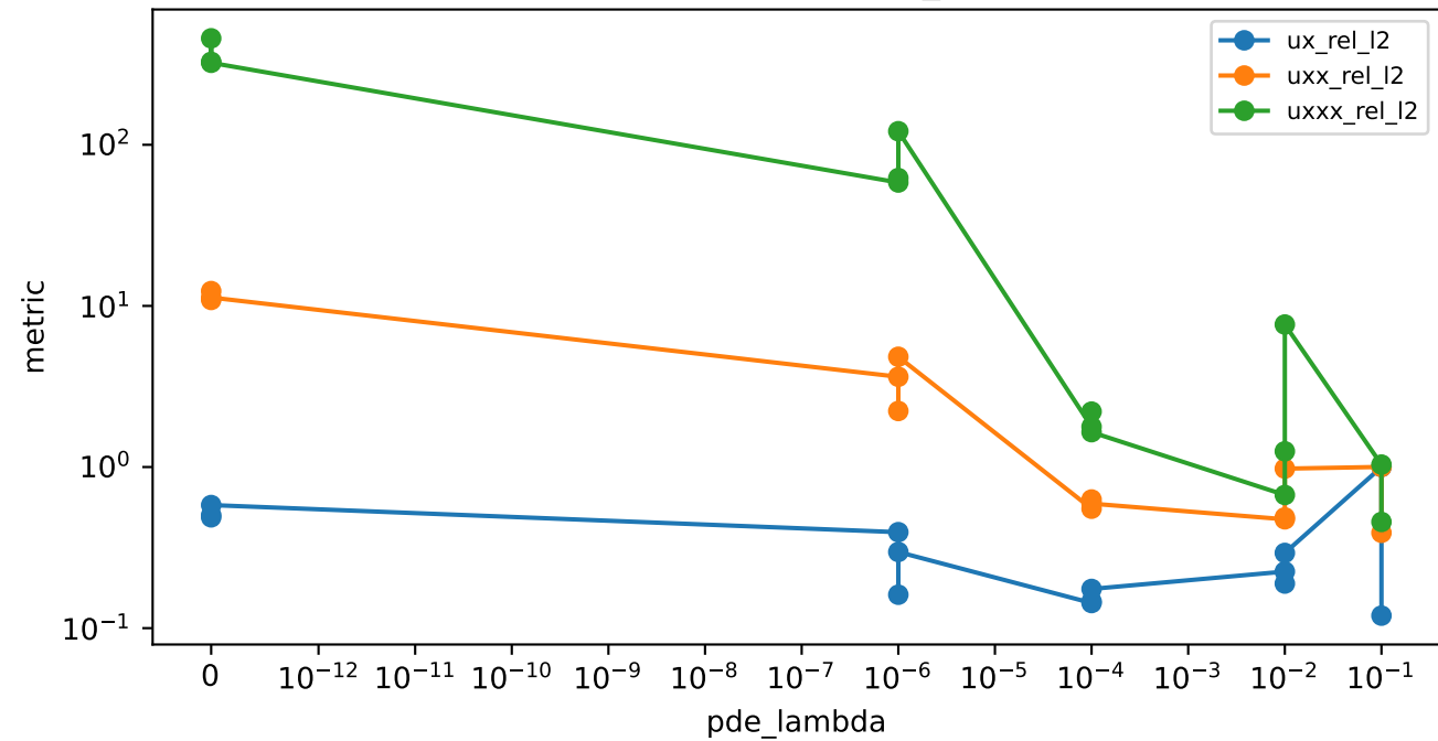
derivative error vs pde_lambda
