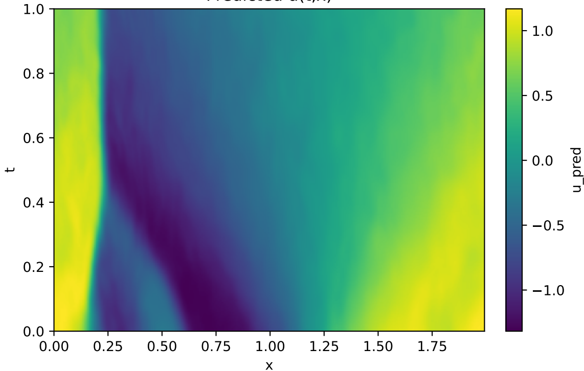
Predicted u(t,x)
