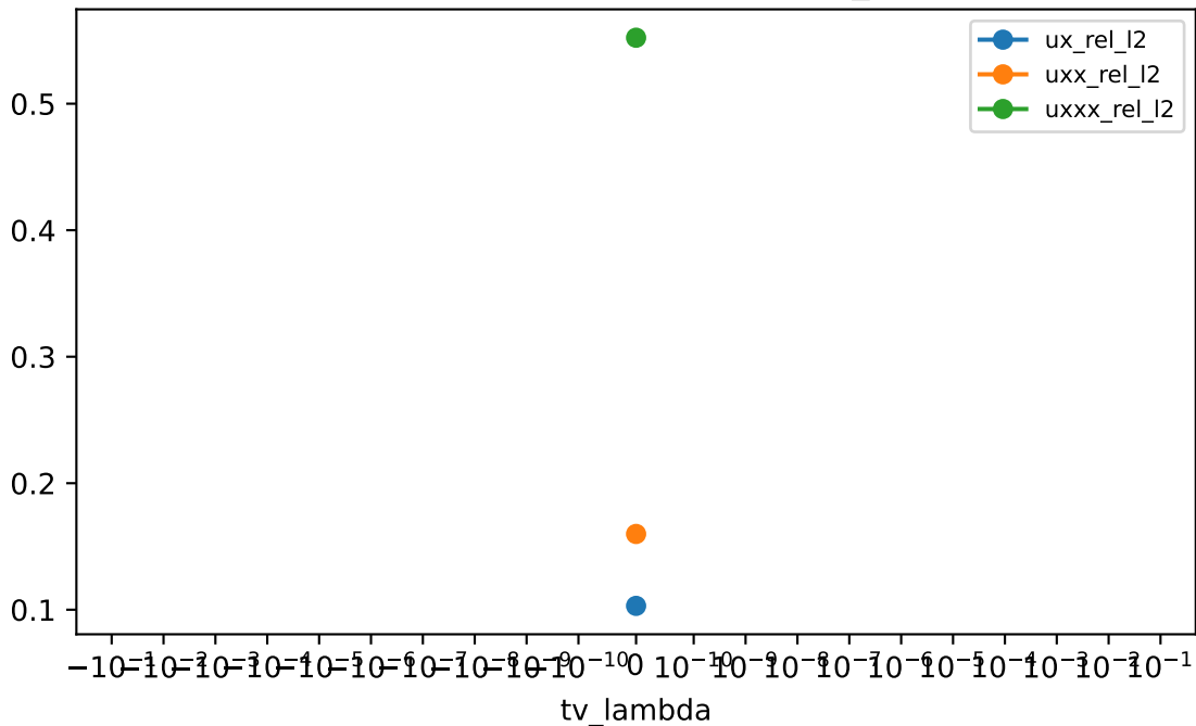
anisotropic: derivative error vs tv_lambda
