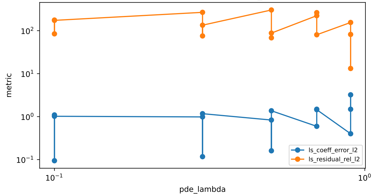
least-squares diagnostics vs pde_lambda
