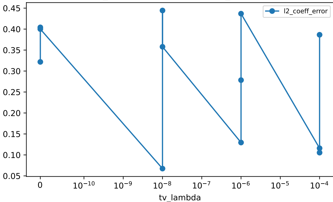
tv_ux: PDE coeff error vs tv_lambda
