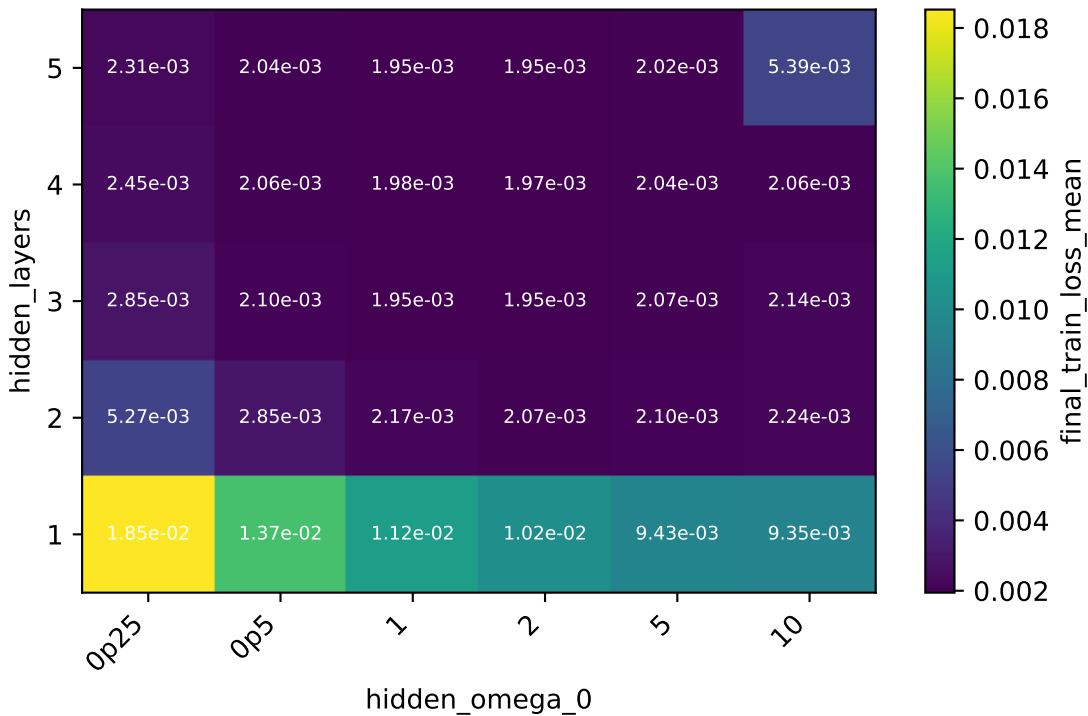
Mean final train loss
