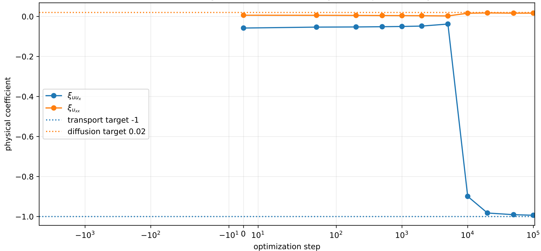
Phase 19B Burgers coefficients over long-horizon joint training
