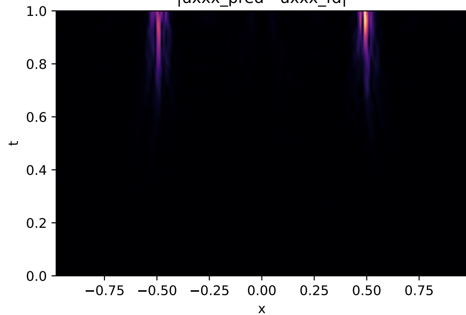
|u_{xxx}_{\text{pred}} - u_{xxx}_{\text{fd}}|
