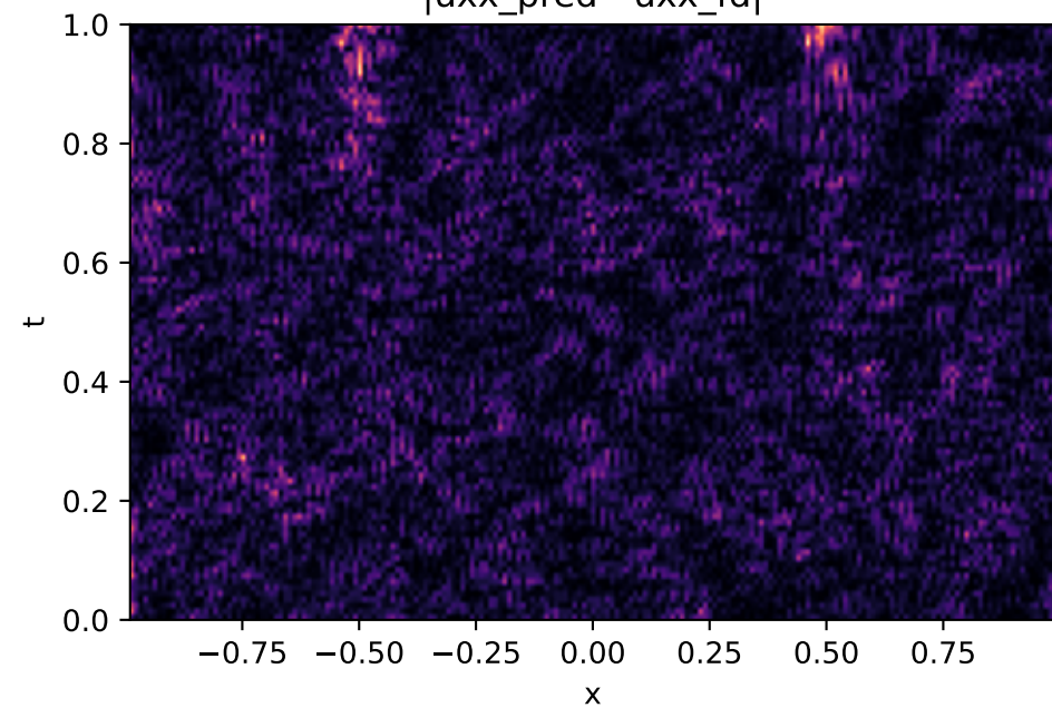
|u_{xx_{\text{pred}}} - u_{xx_{\text{fd}}}|
