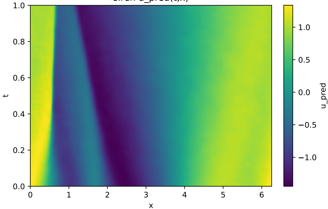
siren u_pred(t,x)
