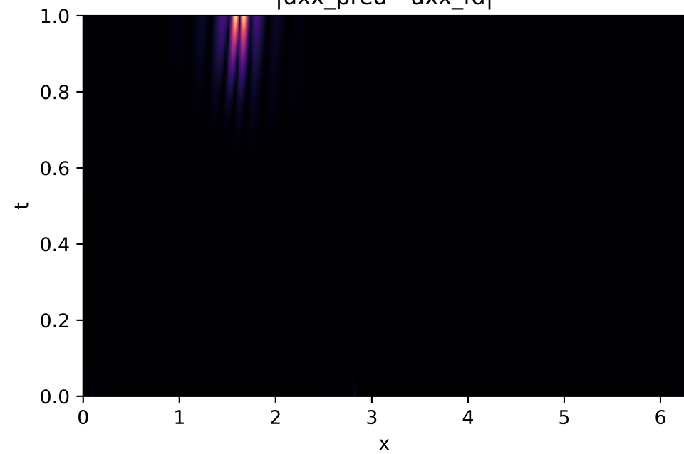
|u_{xx}_{\text{pred}} - u_{xx}_{\text{fd}}|
