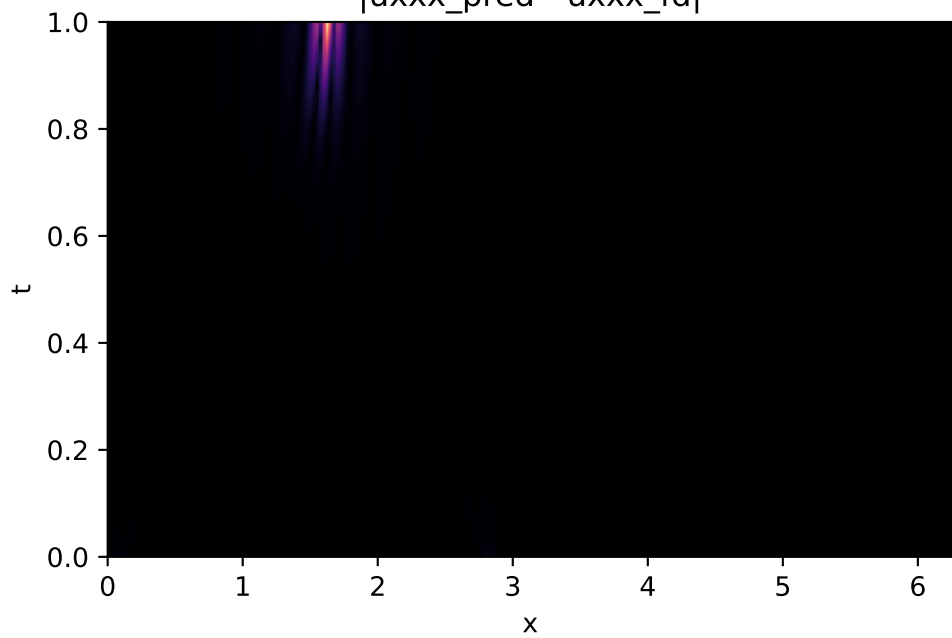
|u_{xxx}_{\text{pred}} - u_{xxx}_{\text{fd}}|
