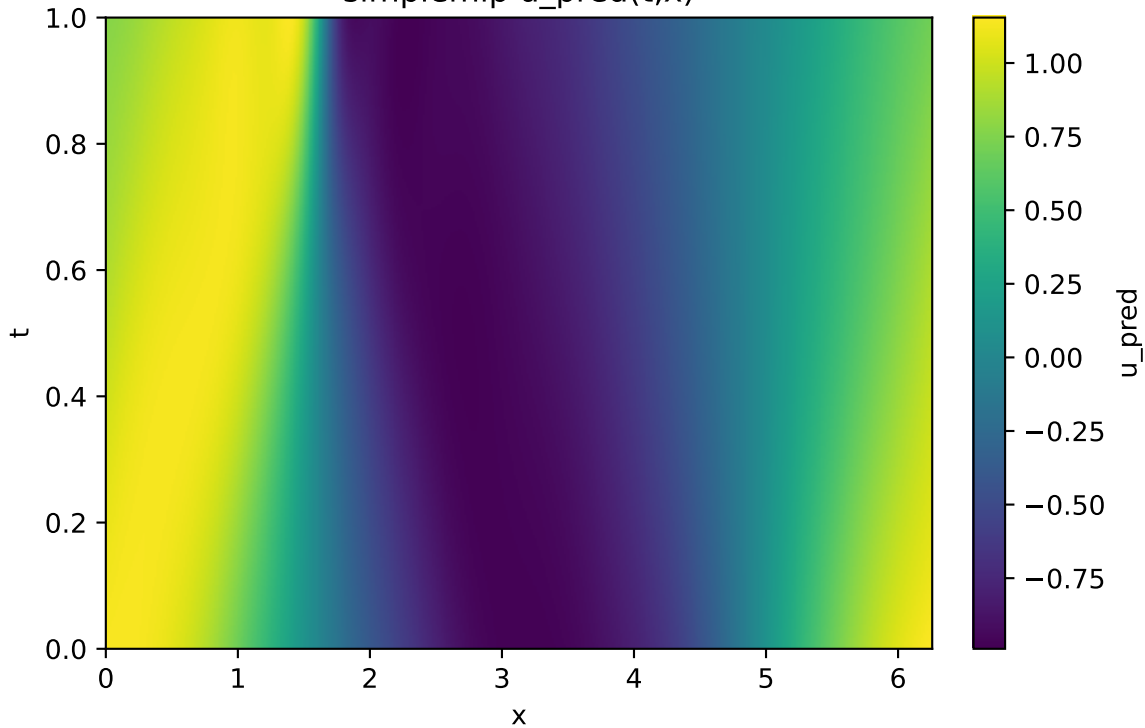
simplemlp u_{\text{pred}}(t,x)
