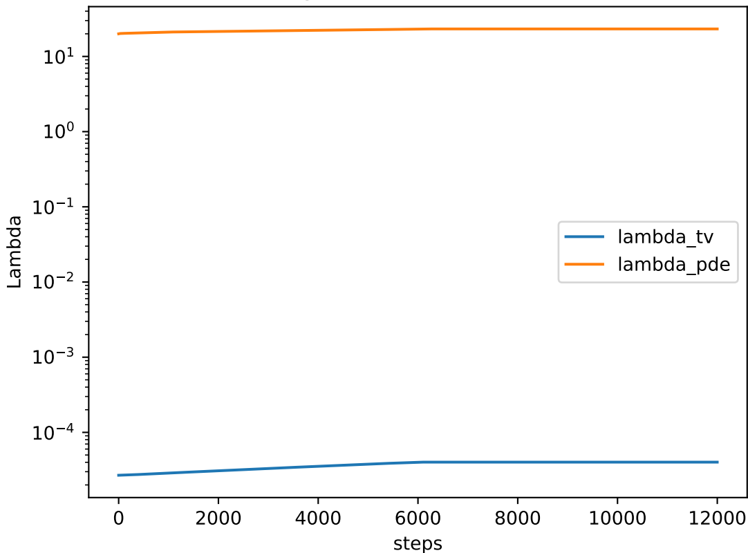
Training Lambda Values (MASKED)
