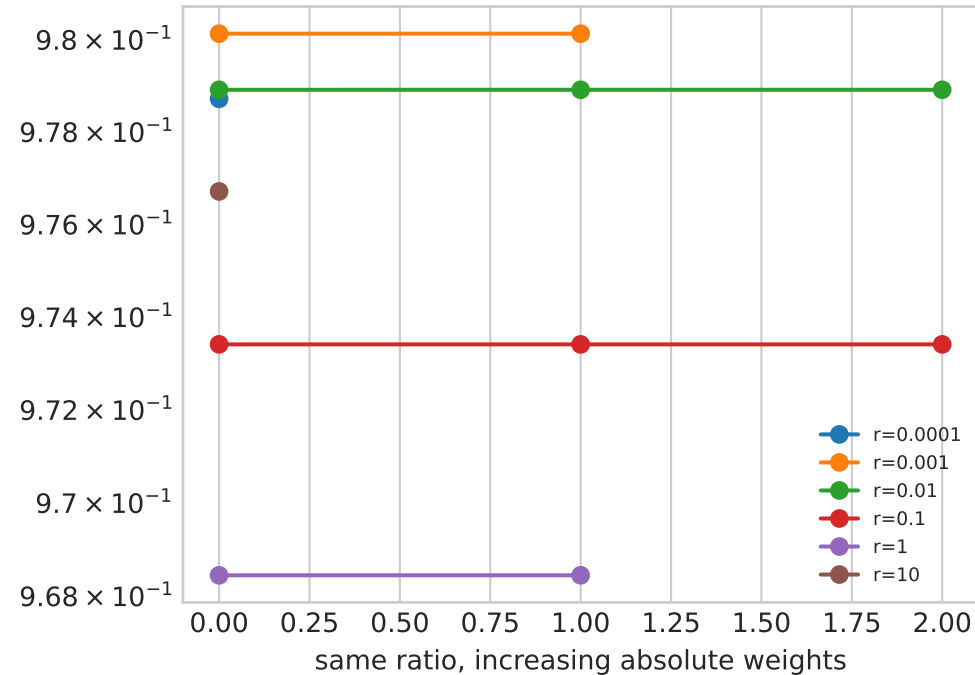
coefficient error
