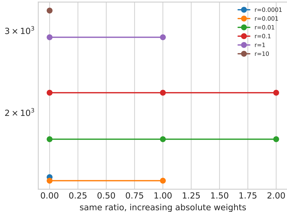
u_xx MSE
