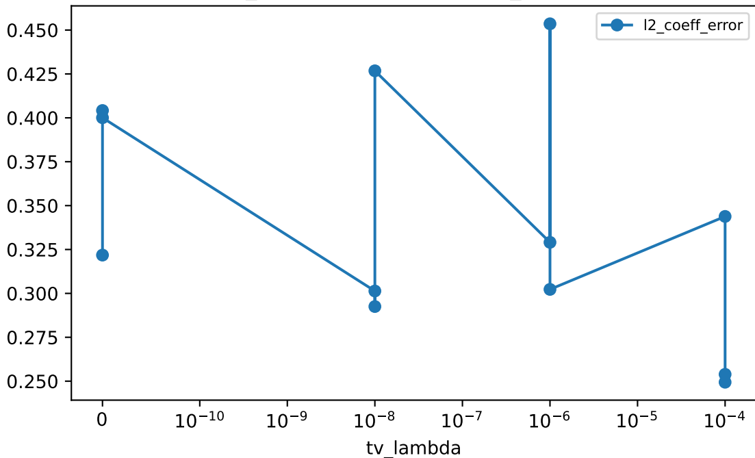
tv_u: PDE coeff error vs tv_lambda
