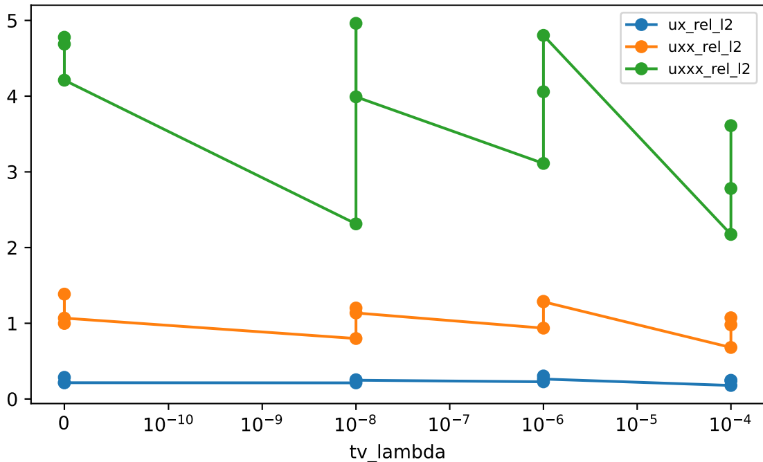
tv_u: derivative error vs tv_lambda
