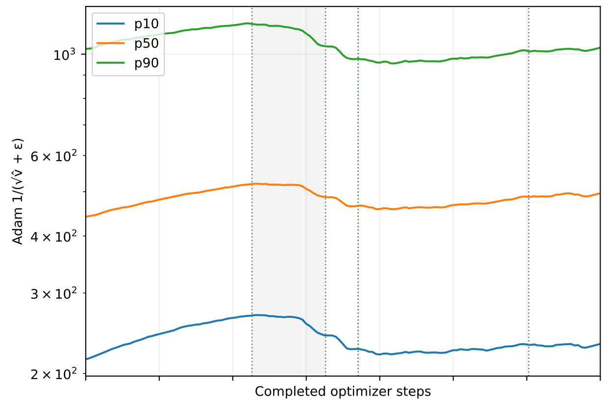
Adam moments and gradient magnitudes: changes versus abrupt events
