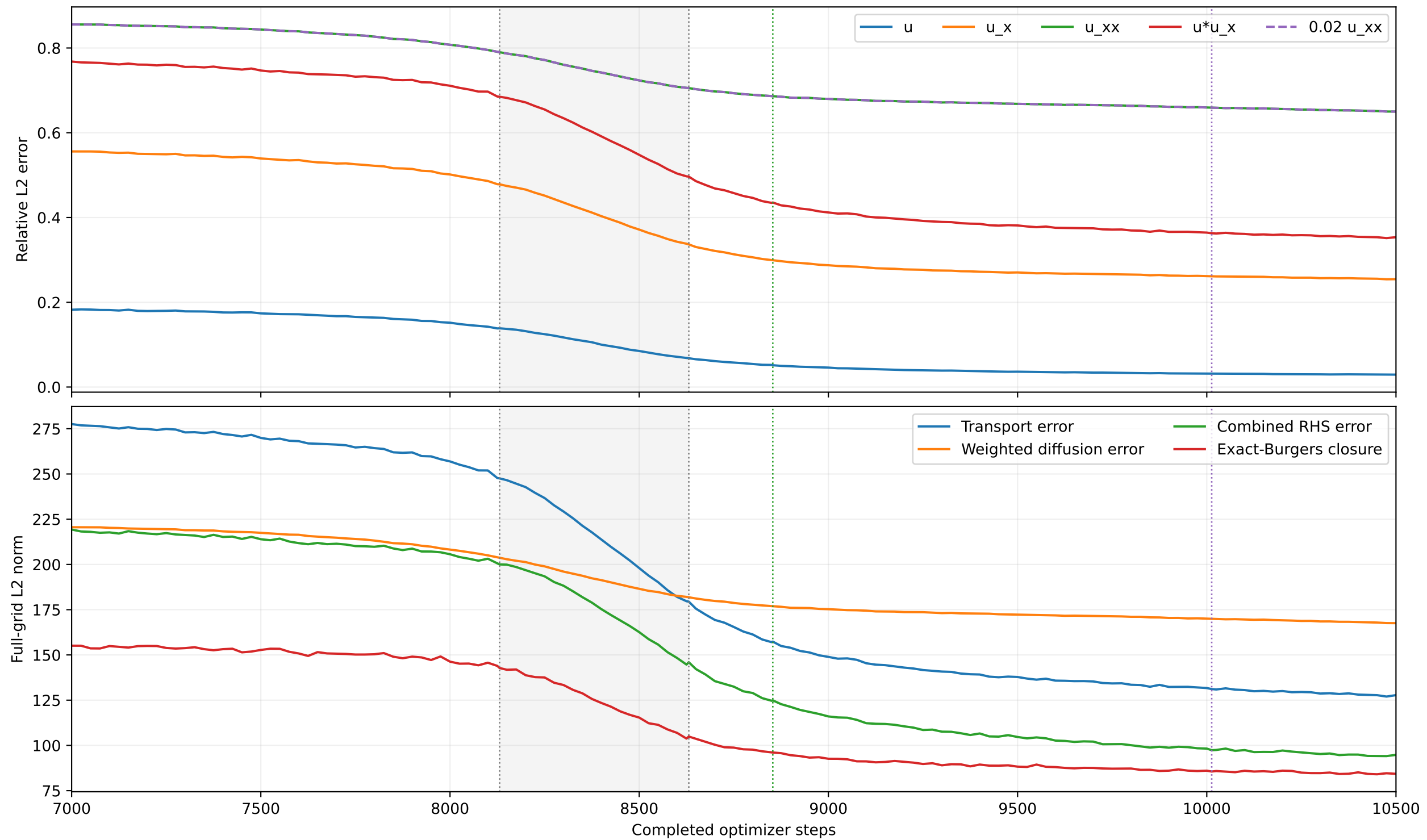
Spatial derivative fidelity and weighted error cancellation
