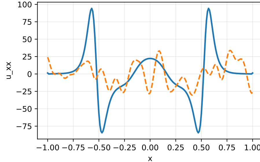
u_xx at t=0
