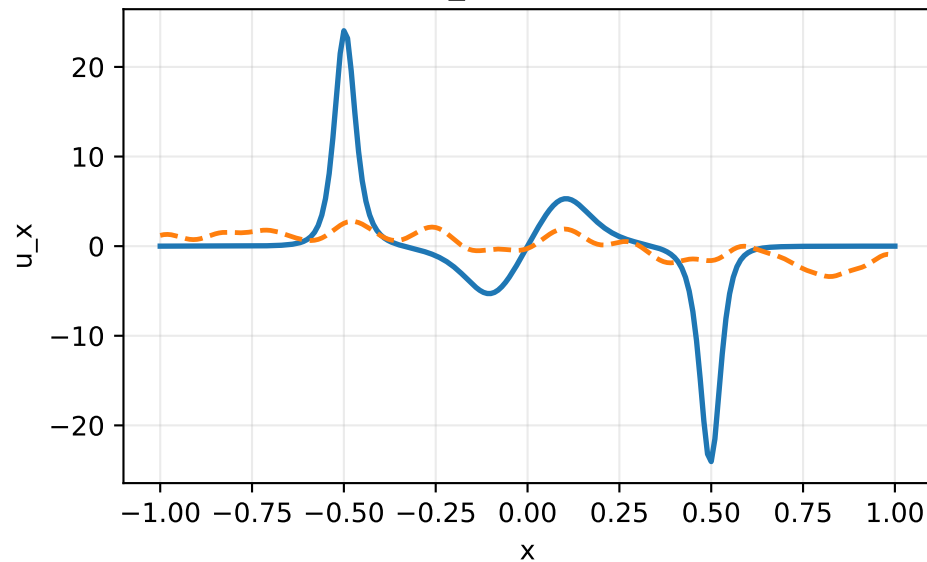
u_x at t=0.5
