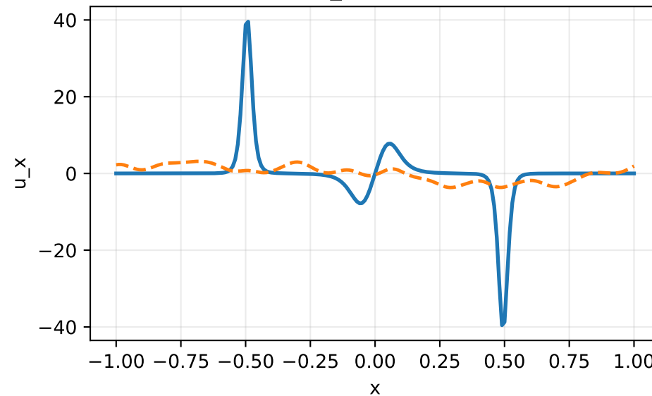
u_x at t=1
