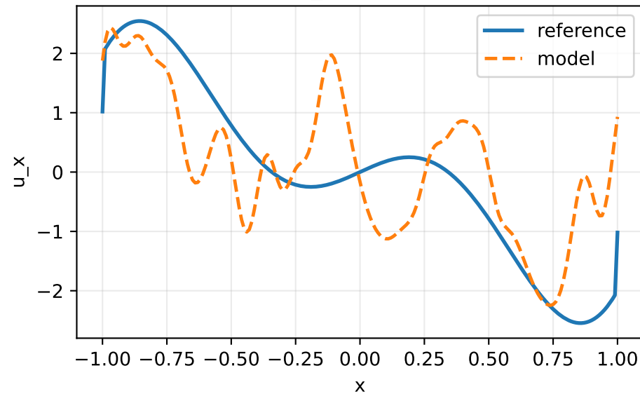
u_x at t=0.5
