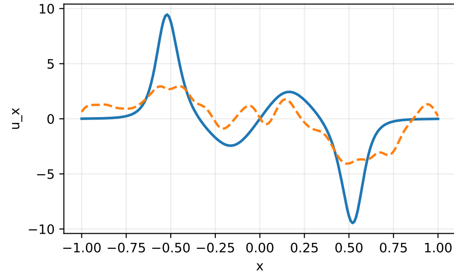
u_x at t=0
