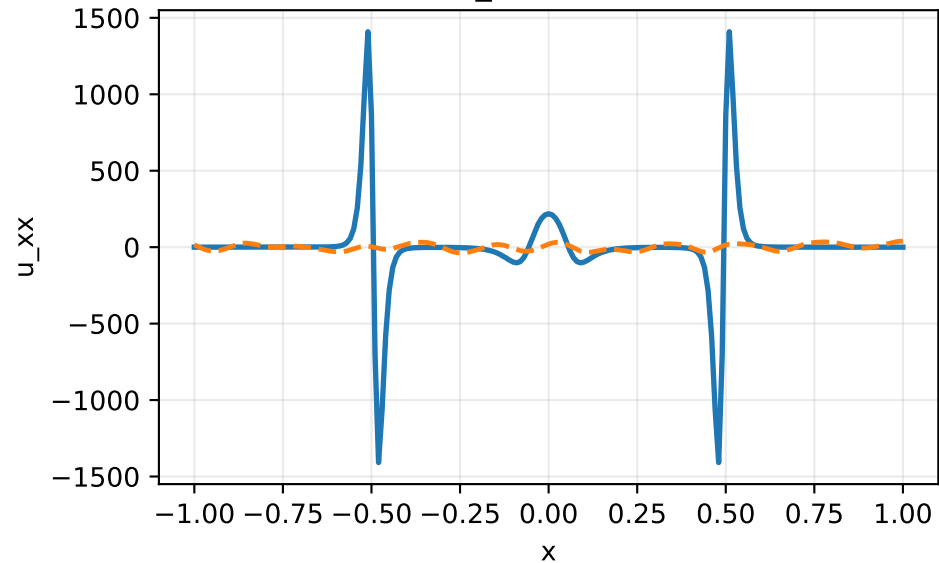
u_xx at t=1
