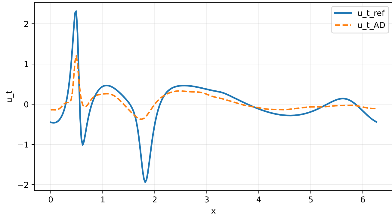
u_t at t=0.25
