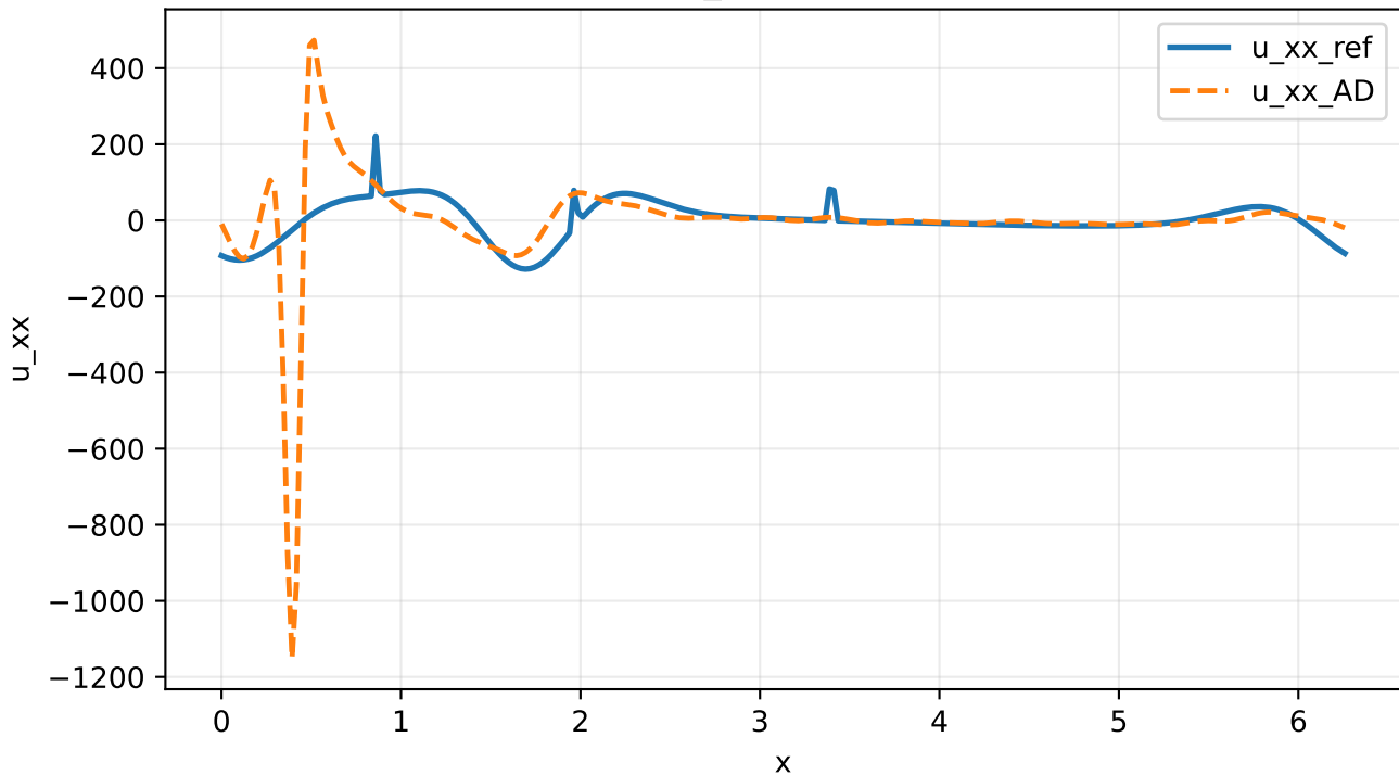
u_{xx} at t=0
