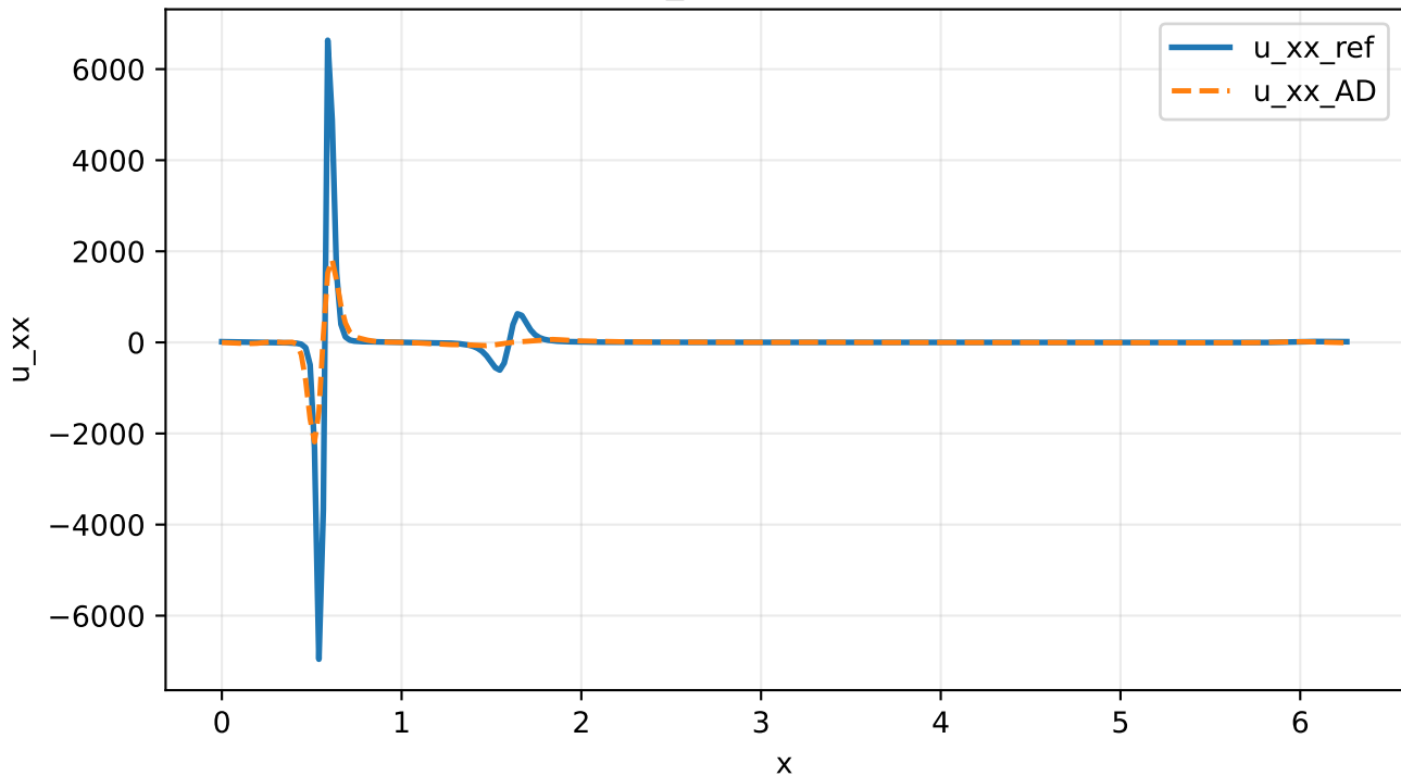
u_{xx} at t=0.502
