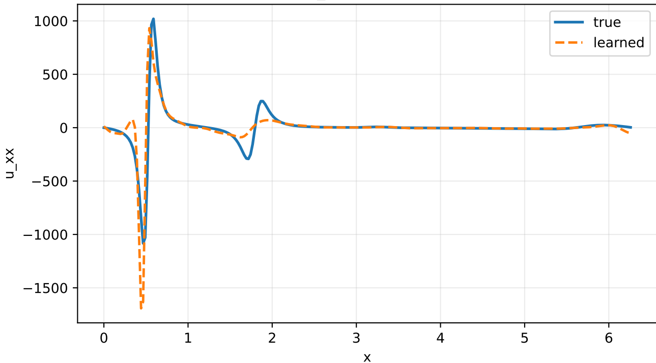
u_{xx} at t=0.25
