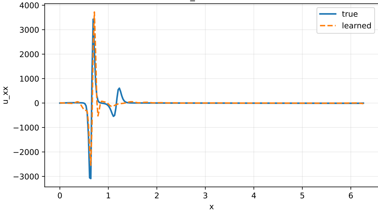
u_xx at t=1
